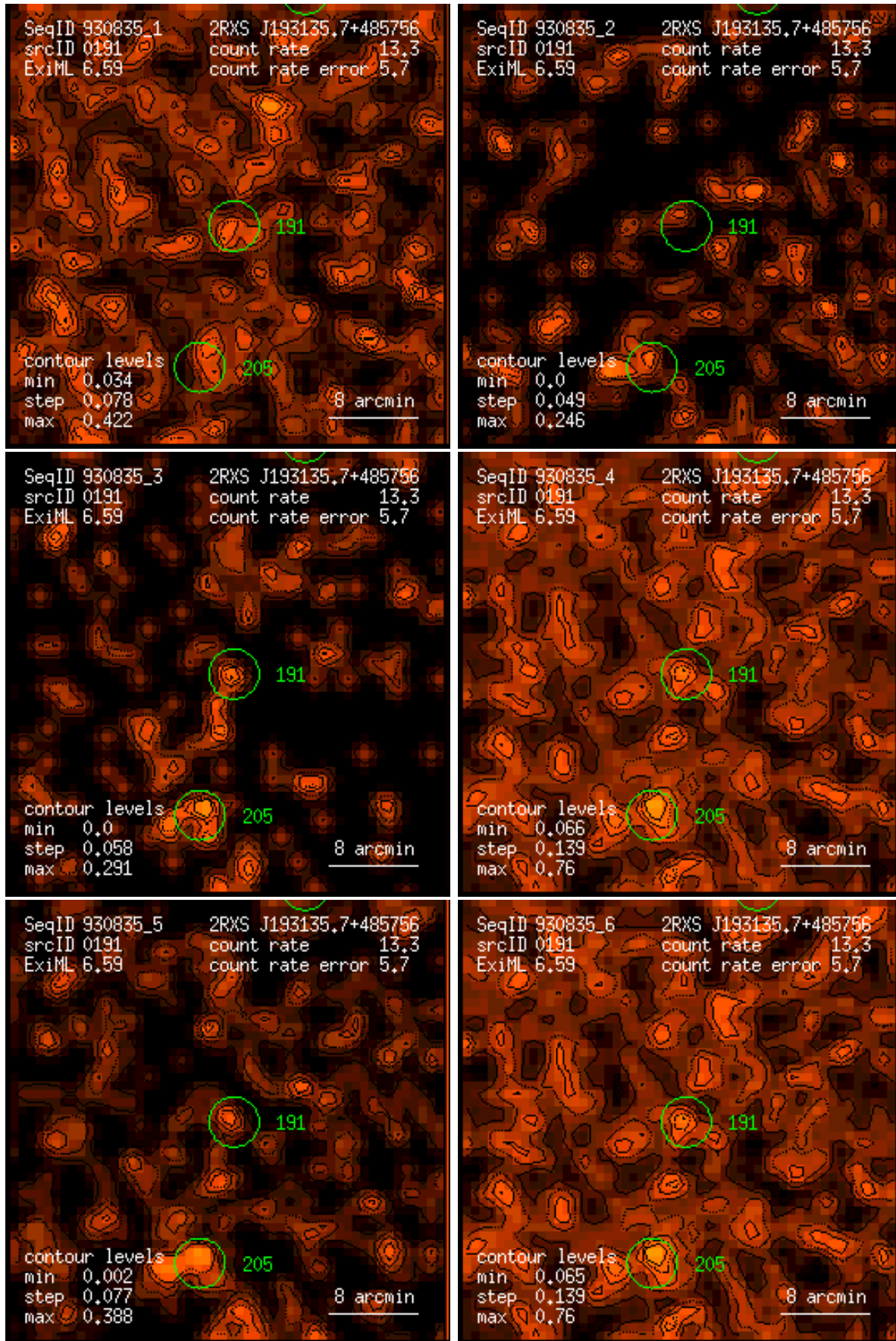
Figure 191: RASS 930835: detection 0191: band rate images, Gaussian filter: (1) PSPC channels 11 – 41, (2) 52 – 90, (3) 91 – 201, (4) 11 – 235, (5) 52 – 201, (6) 11 – 201. Broad band rates in counts/ks. Band rate contour levels in counts/ks/arcmin 2 .
