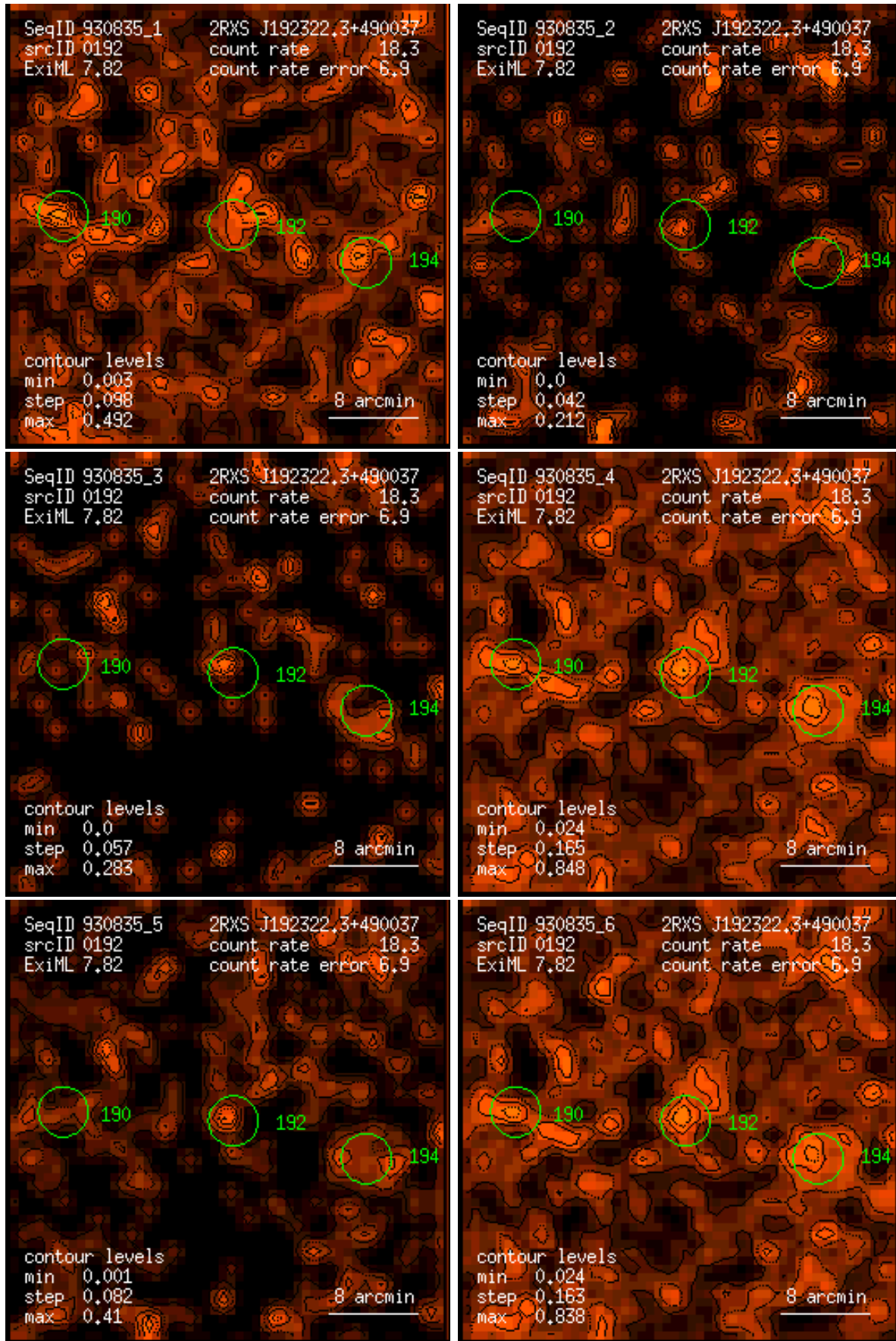
Figure 192: RASS 930835: detection 0192: band rate images, Gaussian filter: (1) PSPC channels 11 – 41, (2) 52 – 90, (3) 91 – 201, (4) 11 – 235, (5) 52 – 201, (6) 11 – 201. Broad band rates in counts/ks. Band rate contour levels in counts/ks/arcmin 2 .
