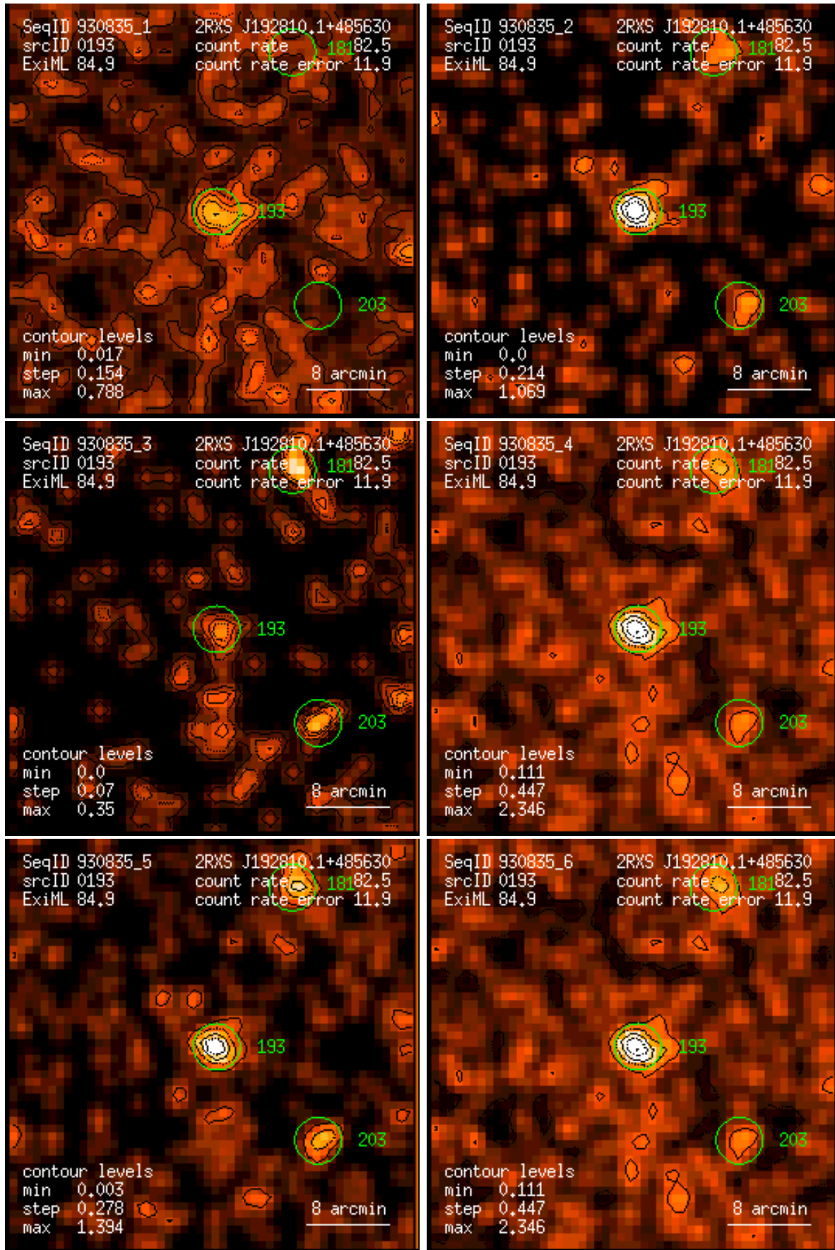
Figure 193: RASS 930835: detection 0193: band rate images, Gaussian filter: (1) PSPC channels 11 – 41, (2) 52 – 90, (3) 91 – 201, (4) 11 – 235, (5) 52 – 201, (6) 11 – 201. Broad band rates in counts/ks. Band rate contour levels in counts/ks/arcmin 2 .
