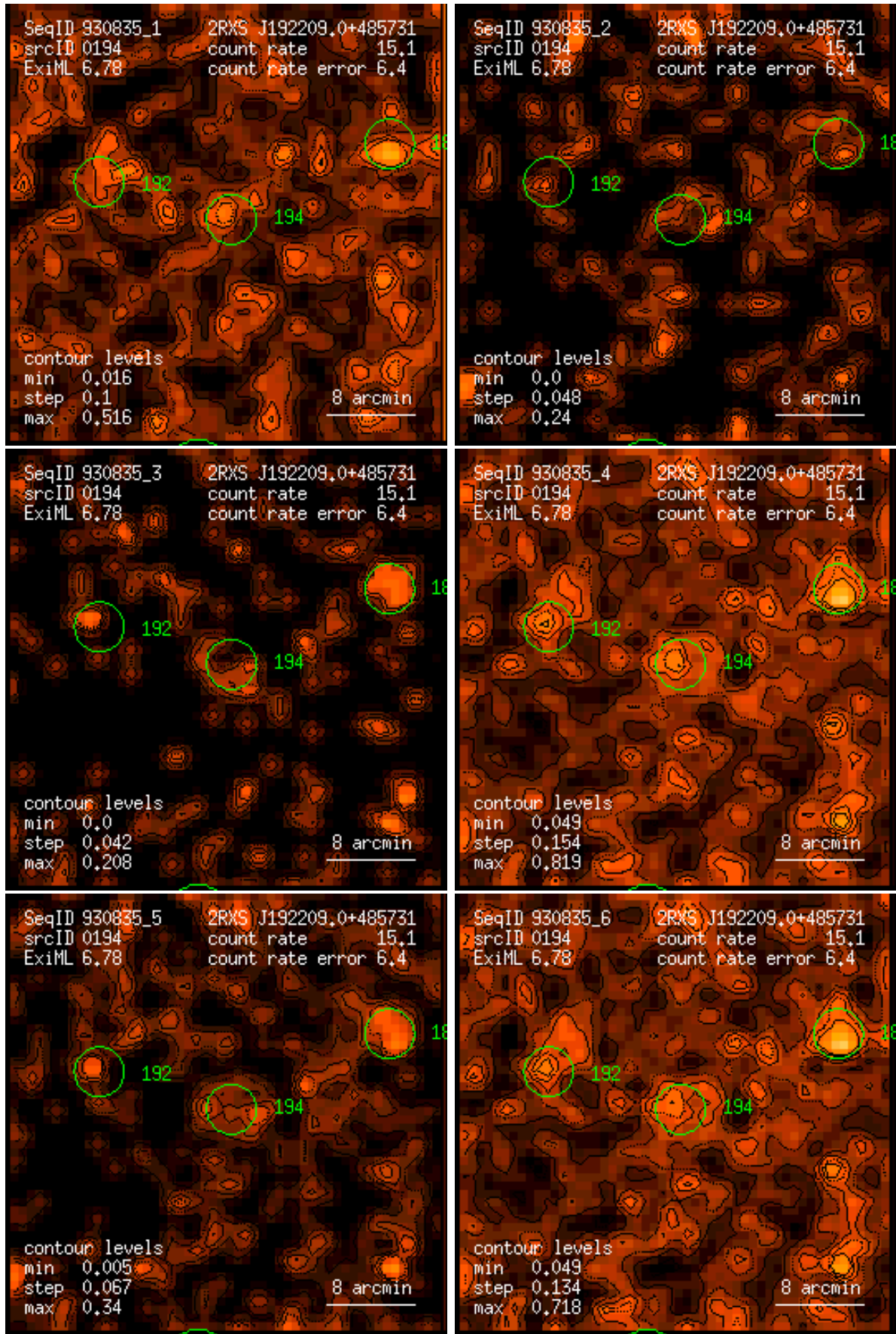
Figure 194: RASS 930835: detection 0194: band rate images, Gaussian filter: (1) PSPC channels 11 – 41, (2) 52 – 90, (3) 91 – 201, (4) 11 – 235, (5) 52 – 201, (6) 11 – 201. Broad band rates in counts/ks. Band rate contour levels in counts/ks/arcmin 2 .
