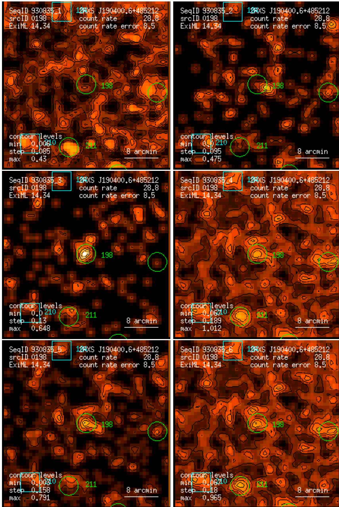
Figure 198: RASS 930835: detection 0198: band rate images, Gaussian filter: (1) PSPC channels 11 – 41, (2) 52 – 90, (3) 91 – 201, (4) 11 – 235, (5) 52 – 201, (6) 11 – 201. Broad band rates in counts/ks. Band rate contour levels in counts/ks/arcmin 2 .
