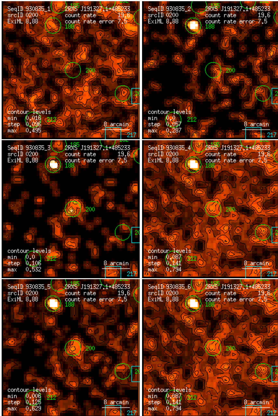
Figure 200: RASS 930835: detection 0200: band rate images, Gaussian filter: (1) PSPC channels 11 – 41, (2) 52 – 90, (3) 91 – 201, (4) 11 – 235, (5) 52 – 201, (6) 11 – 201. Broad band rates in counts/ks. Band rate contour levels in counts/ks/arcmin 2 .
