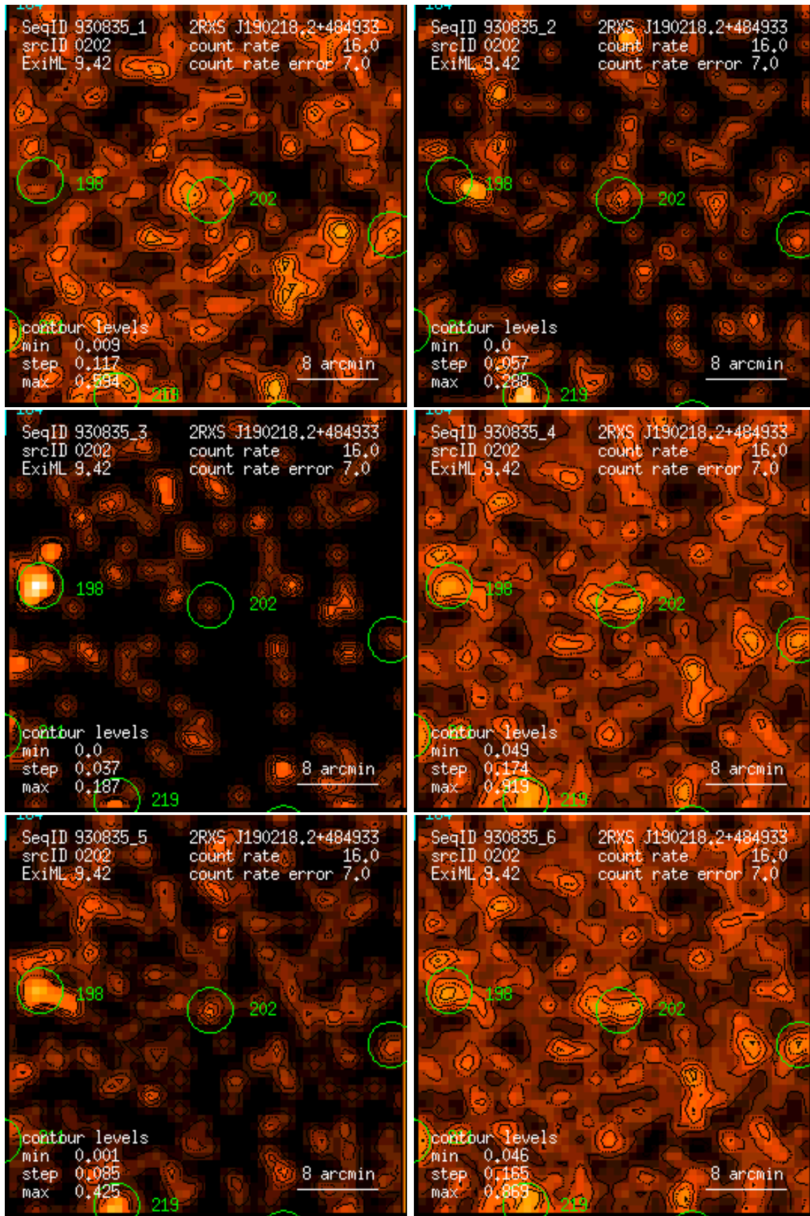
Figure 202: RASS 930835: detection 0202: band rate images, Gaussian filter: (1) PSPC channels 11 – 41, (2) 52 – 90, (3) 91 – 201, (4) 11 – 235, (5) 52 – 201, (6) 11 – 201. Broad band rates in counts/ks. Band rate contour levels in counts/ks/arcmin 2 .
