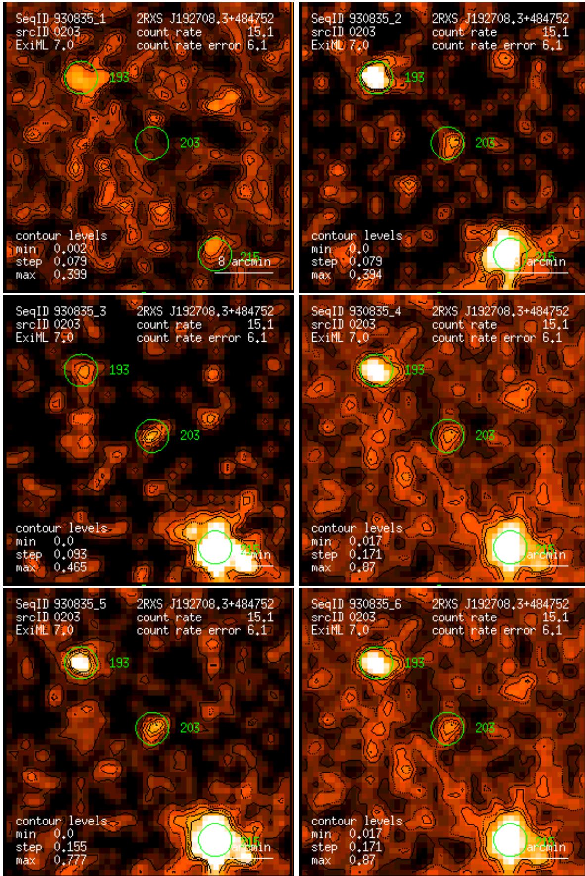
Figure 203: RASS 930835: detection 0203: band rate images, Gaussian filter: (1) PSPC channels 11 – 41, (2) 52 – 90, (3) 91 – 201, (4) 11 – 235, (5) 52 – 201, (6) 11 – 201. Broad band rates in counts/ks. Band rate contour levels in counts/ks/arcmin 2 .
