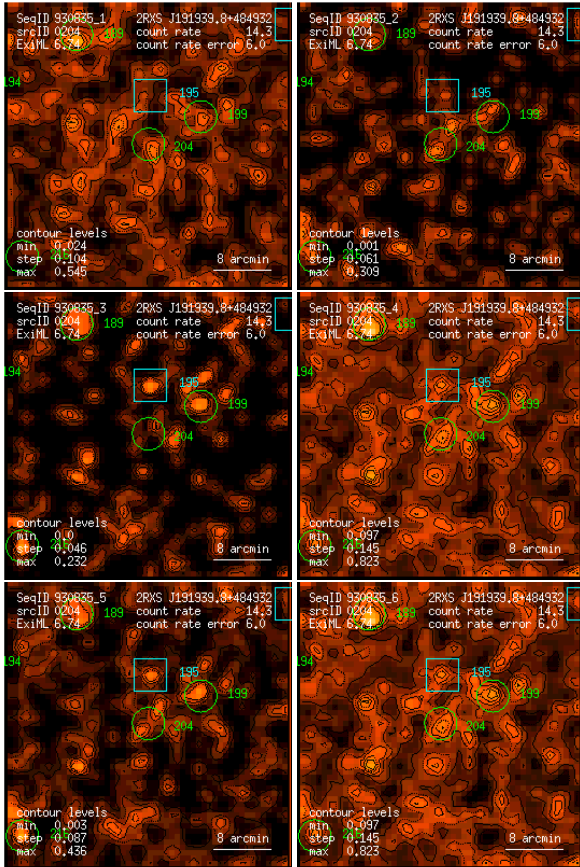
Figure 204: RASS 930835: detection 0204: band rate images, Gaussian filter: (1) PSPC channels 11 – 41, (2) 52 – 90, (3) 91 – 201, (4) 11 – 235, (5) 52 – 201, (6) 11 – 201. Broad band rates in counts/ks. Band rate contour levels in counts/ks/arcmin 2 .
