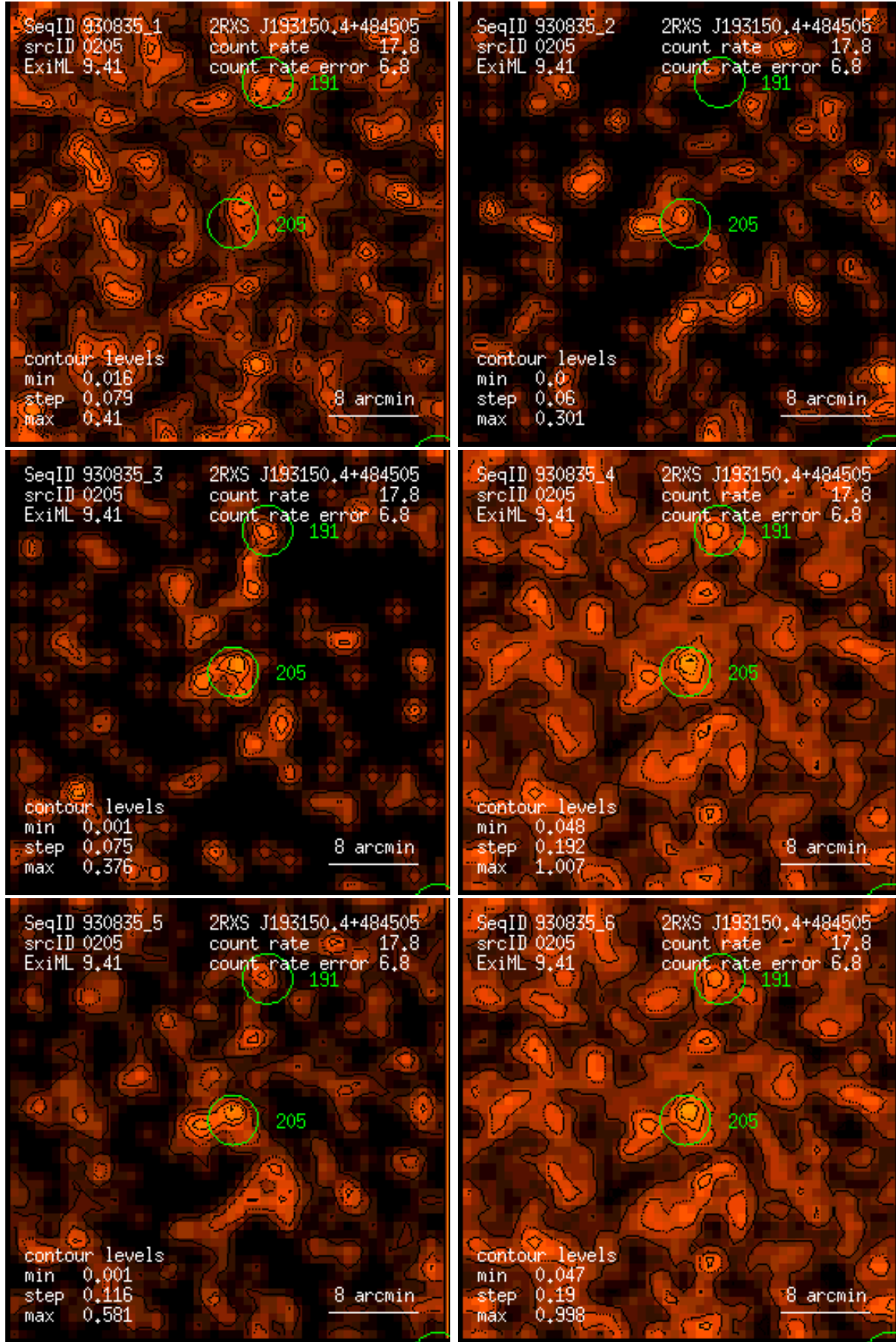
Figure 205: RASS 930835: detection 0205: band rate images, Gaussian filter: (1) PSPC channels 11 – 41, (2) 52 – 90, (3) 91 – 201, (4) 11 – 235, (5) 52 – 201, (6) 11 – 201. Broad band rates in counts/ks. Band rate contour levels in counts/ks/arcmin 2 .
