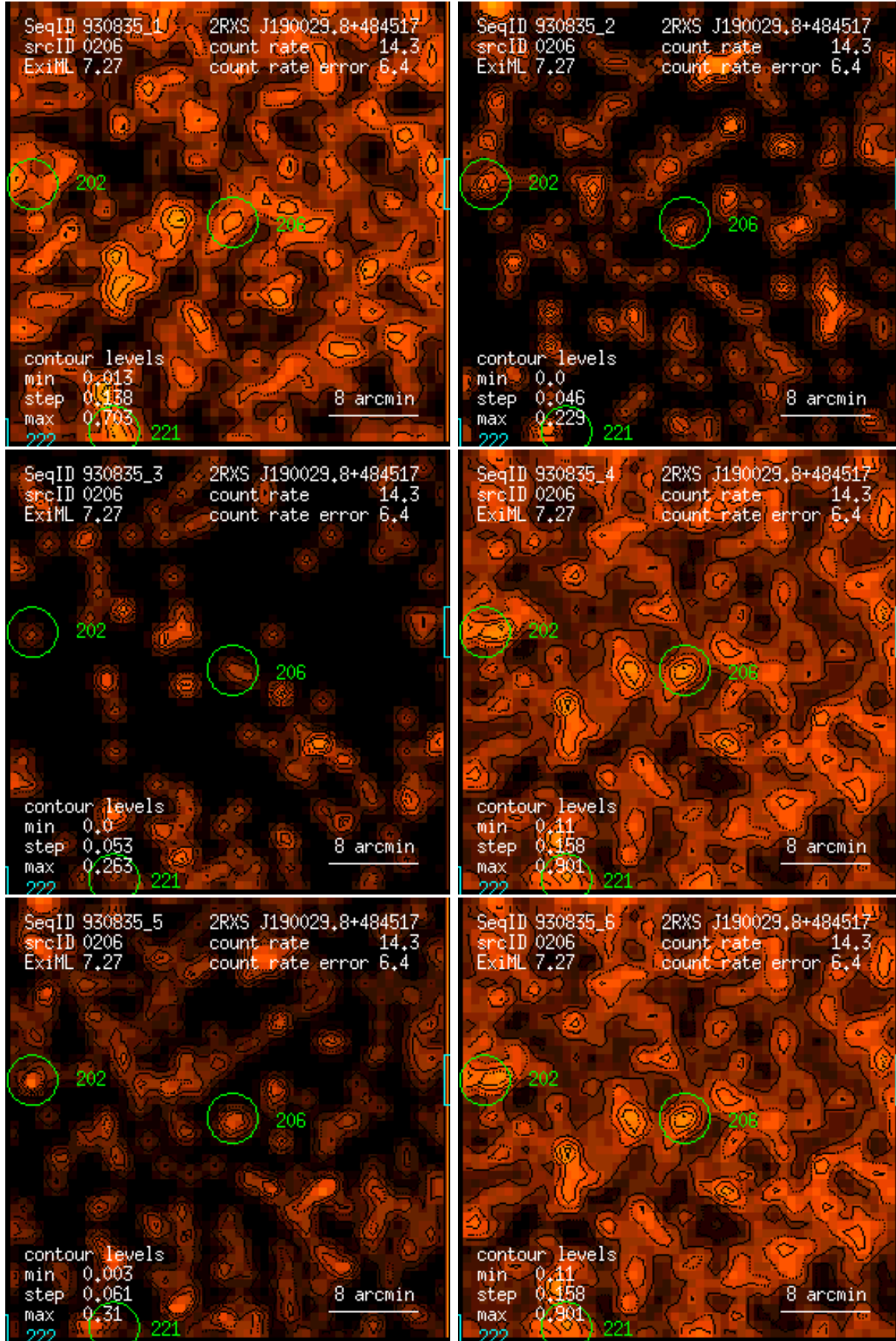
Figure 206: RASS 930835: detection 0206: band rate images, Gaussian filter: (1) PSPC channels 11 – 41, (2) 52 – 90, (3) 91 – 201, (4) 11 – 235, (5) 52 – 201, (6) 11 – 201. Broad band rates in counts/ks. Band rate contour levels in counts/ks/arcmin 2 .
