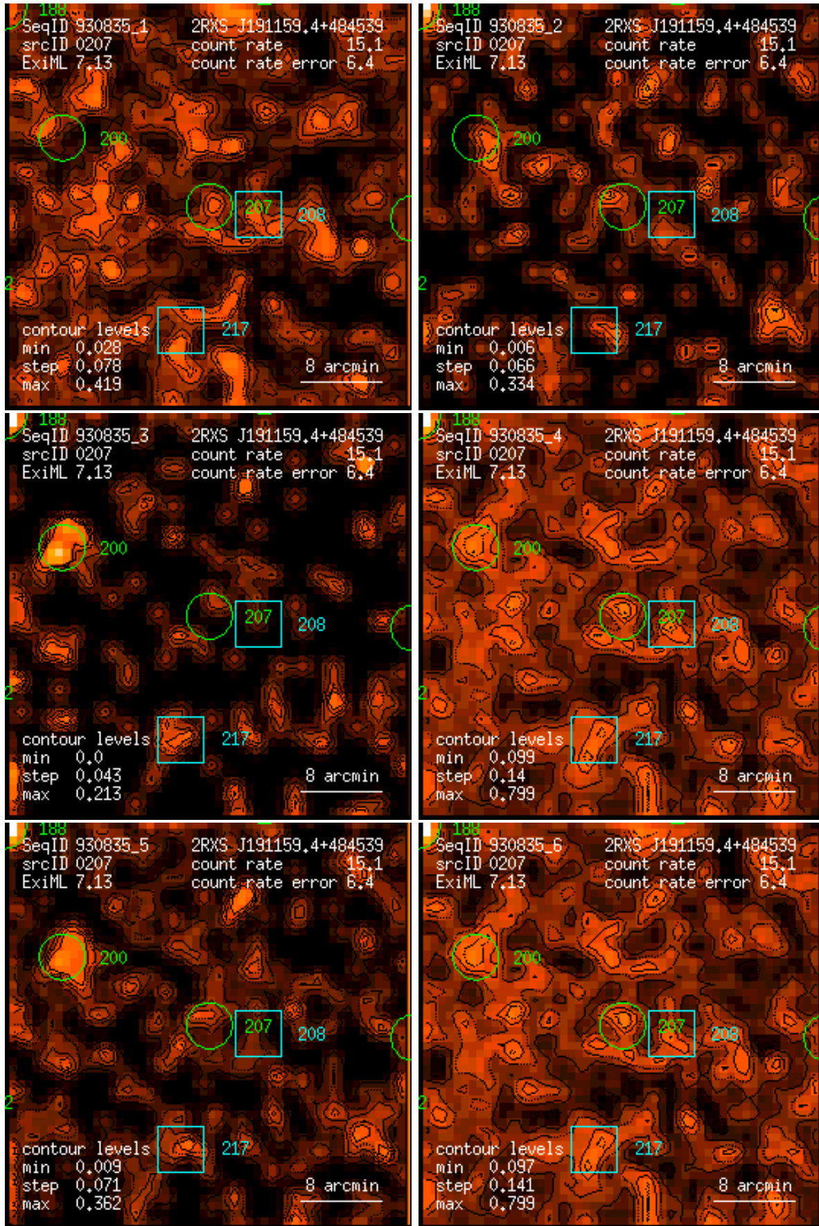
Figure 207: RASS 930835: detection 0207: band rate images, Gaussian filter: (1) PSPC channels 11 – 41, (2) 52 – 90, (3) 91 – 201, (4) 11 – 235, (5) 52 – 201, (6) 11 – 201. Broad band rates in counts/ks. Band rate contour levels in counts/ks/arcmin 2 .
