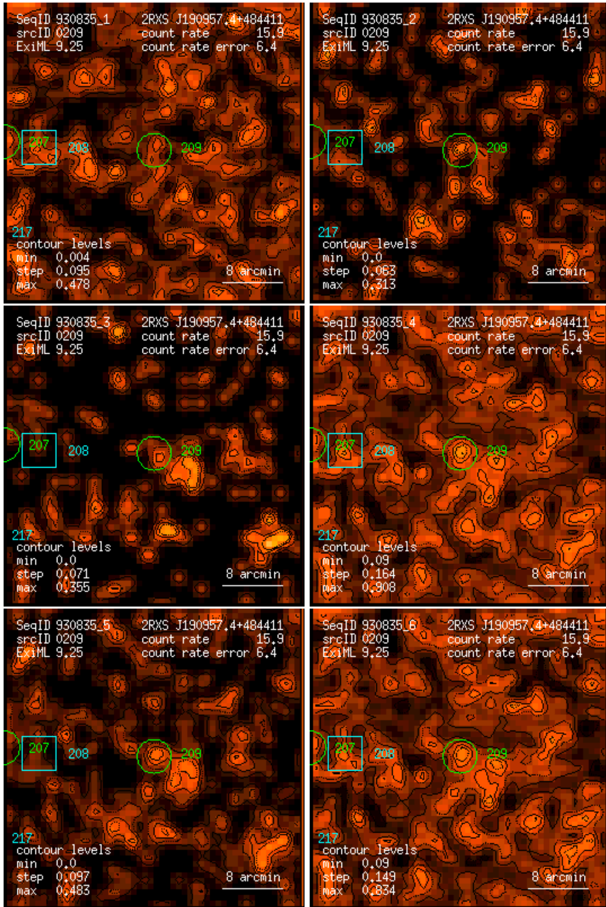
Figure 209: RASS 930835: detection 0209: band rate images, Gaussian filter: (1) PSPC channels 11 – 41, (2) 52 – 90, (3) 91 – 201, (4) 11 – 235, (5) 52 – 201, (6) 11 – 201. Broad band rates in counts/ks. Band rate contour levels in counts/ks/arcmin 2 .
