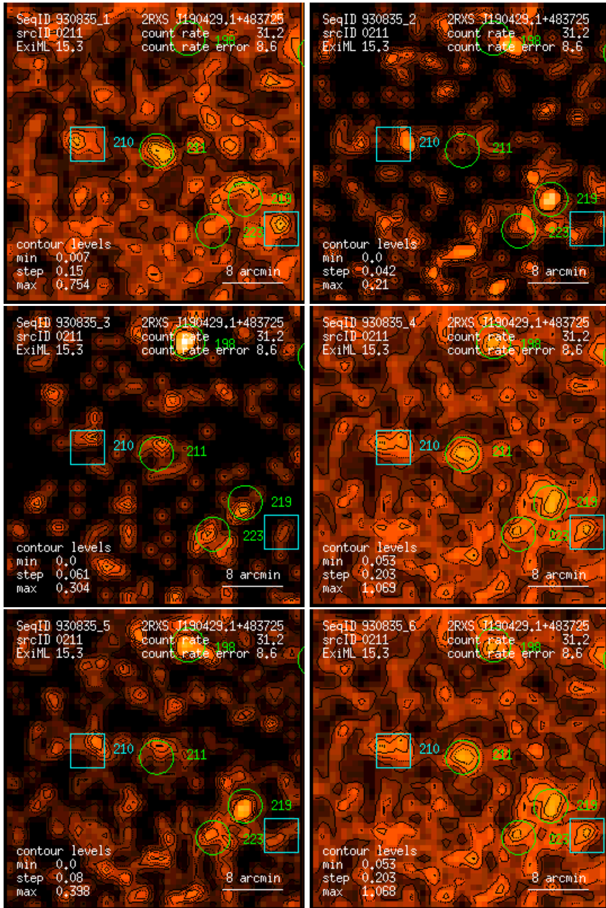
Figure 211: RASS 930835: detection 0211: band rate images, Gaussian filter: (1) PSPC channels 11 – 41, (2) 52 – 90, (3) 91 – 201, (4) 11 – 235, (5) 52 – 201, (6) 11 – 201. Broad band rates in counts/ks. Band rate contour levels in counts/ks/arcmin 2 .
