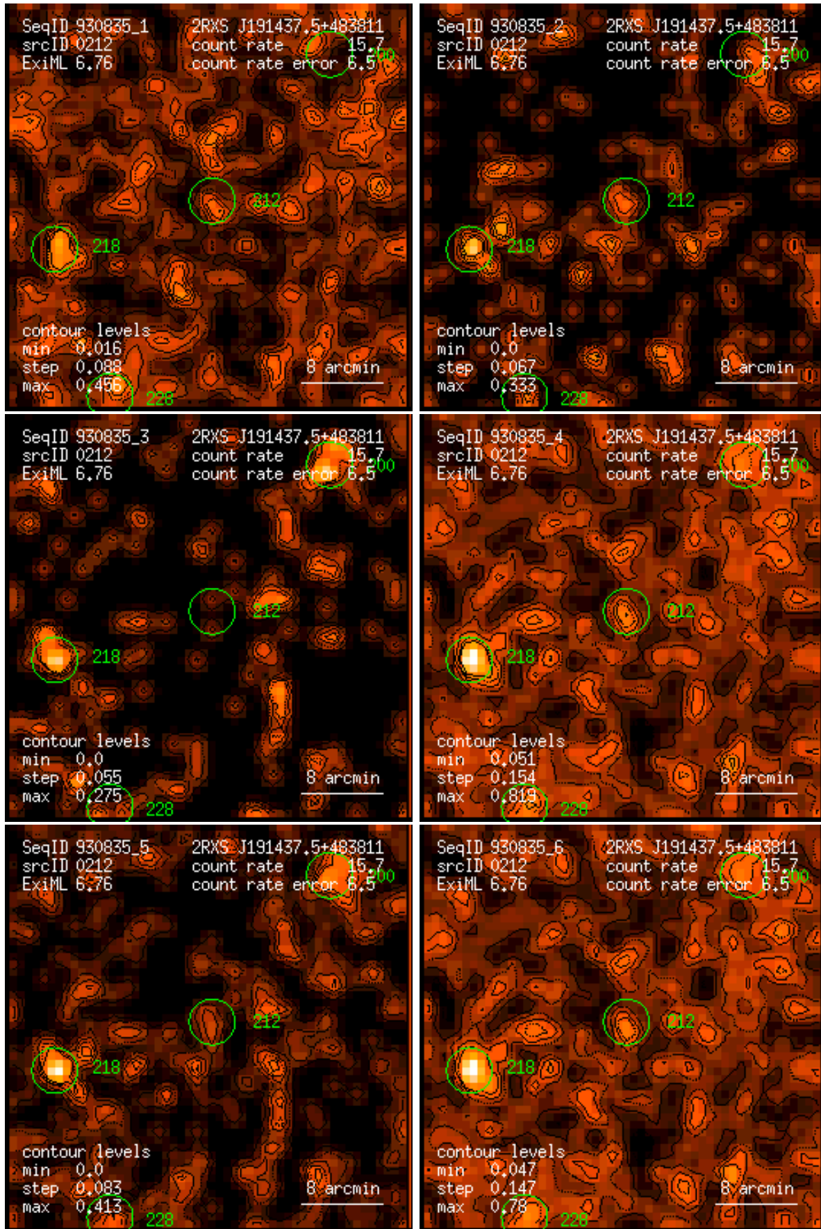
Figure 212: RASS 930835: detection 0212: band rate images, Gaussian filter: (1) PSPC channels 11 – 41, (2) 52 – 90, (3) 91 – 201, (4) 11 – 235, (5) 52 – 201, (6) 11 – 201. Broad band rates in counts/ks. Band rate contour levels in counts/ks/arcmin 2 .
