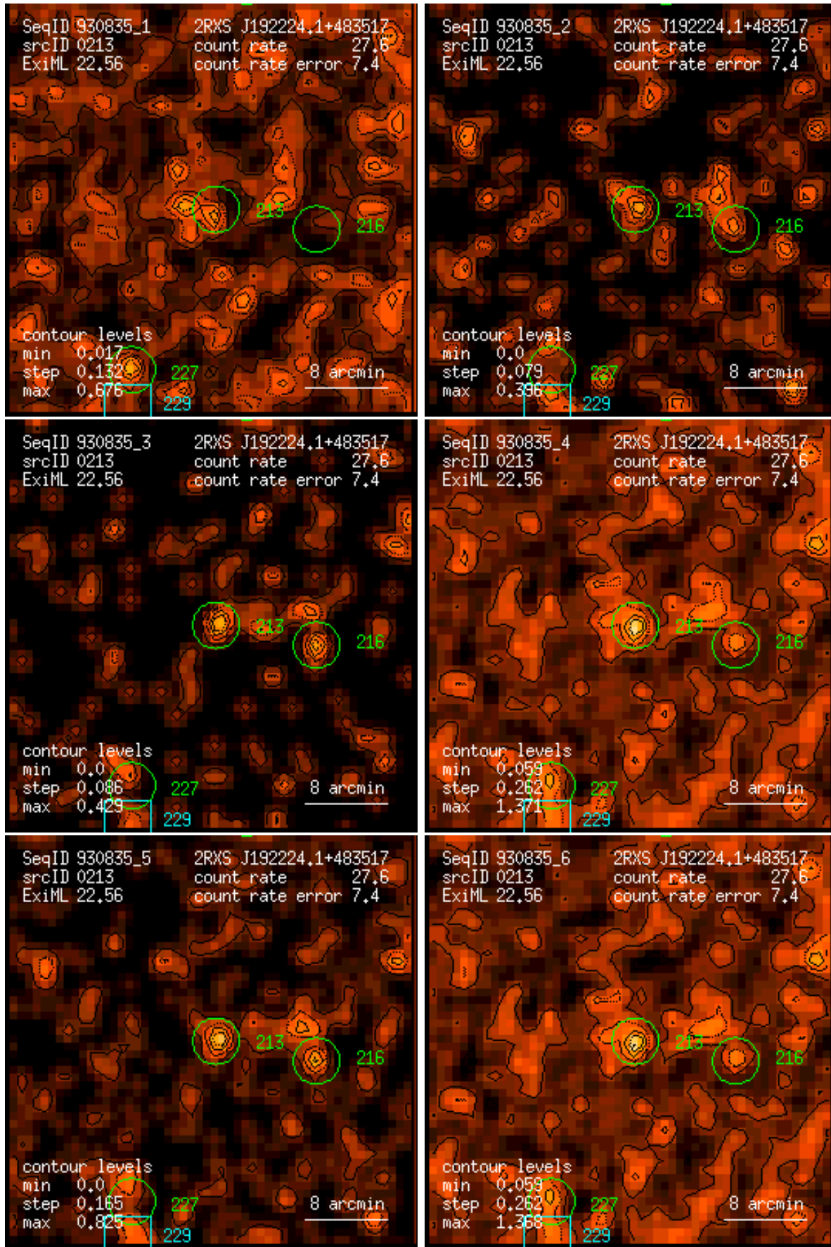
Figure 213: RASS 930835: detection 0213: band rate images, Gaussian filter: (1) PSPC channels 11 – 41, (2) 52 – 90, (3) 91 – 201, (4) 11 – 235, (5) 52 – 201, (6) 11 – 201. Broad band rates in counts/ks. Band rate contour levels in counts/ks/arcmin 2 .
