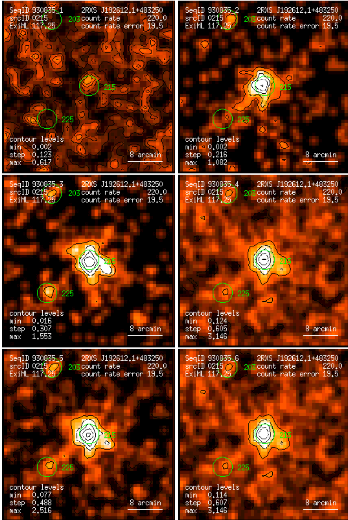
Figure 215: RASS 930835: detection 0215: band rate images, Gaussian filter: (1) PSPC channels 11 – 41, (2) 52 – 90, (3) 91 – 201, (4) 11 – 235, (5) 52 – 201, (6) 11 – 201. Broad band rates in counts/ks. Band rate contour levels in counts/ks/arcmin 2 .
