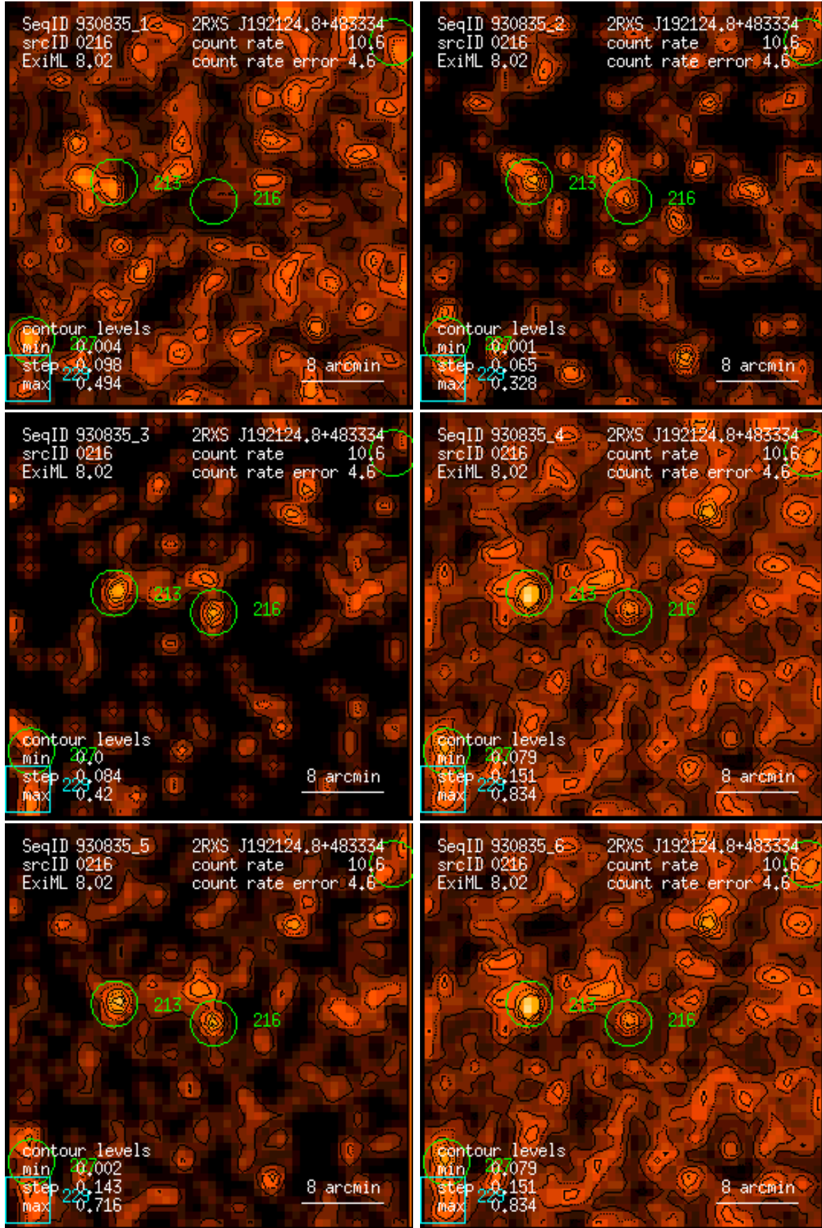
Figure 216: RASS 930835: detection 0216: band rate images, Gaussian filter: (1) PSPC channels 11 – 41, (2) 52 – 90, (3) 91 – 201, (4) 11 – 235, (5) 52 – 201, (6) 11 – 201. Broad band rates in counts/ks. Band rate contour levels in counts/ks/arcmin 2 .
