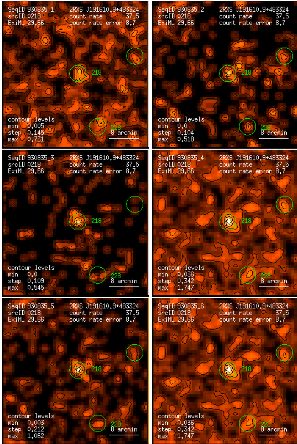
Figure 218: RASS 930835: detection 0218: band rate images, Gaussian filter: (1) PSPC channels 11 – 41, (2) 52 – 90, (3) 91 – 201, (4) 11 – 235, (5) 52 – 201, (6) 11 – 201. Broad band rates in counts/ks. Band rate contour levels in counts/ks/arcmin 2 .
