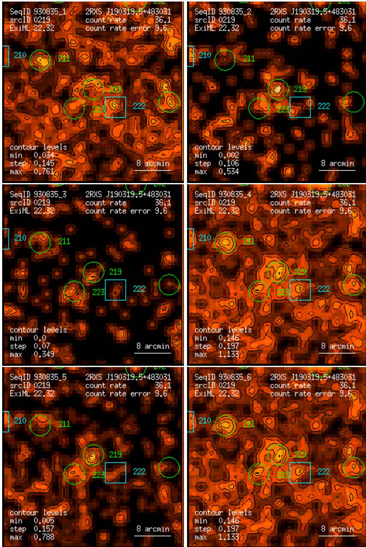
Figure 219: RASS 930835: detection 0219: band rate images, Gaussian filter: (1) PSPC channels 11 – 41, (2) 52 – 90, (3) 91 – 201, (4) 11 – 235, (5) 52 – 201, (6) 11 – 201. Broad band rates in counts/ks. Band rate contour levels in counts/ks/arcmin 2 .
