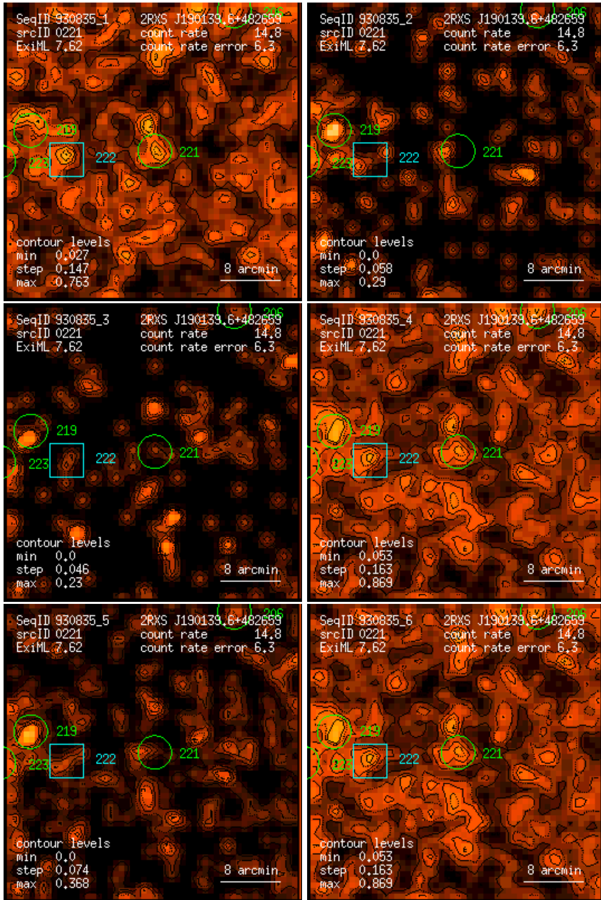
Figure 221: RASS 930835: detection 0221: band rate images, Gaussian filter: (1) PSPC channels 11 – 41, (2) 52 – 90, (3) 91 – 201, (4) 11 – 235, (5) 52 – 201, (6) 11 – 201. Broad band rates in counts/ks. Band rate contour levels in counts/ks/arcmin 2 .
