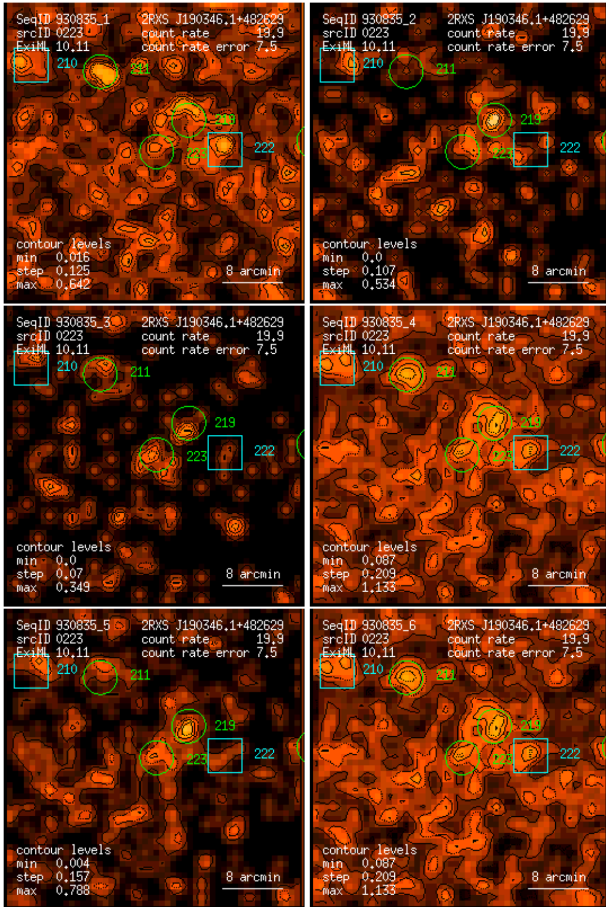
Figure 223: RASS 930835: detection 0223: band rate images, Gaussian filter: (1) PSPC channels 11 – 41, (2) 52 – 90, (3) 91 – 201, (4) 11 – 235, (5) 52 – 201, (6) 11 – 201. Broad band rates in counts/ks. Band rate contour levels in counts/ks/arcmin 2 .
