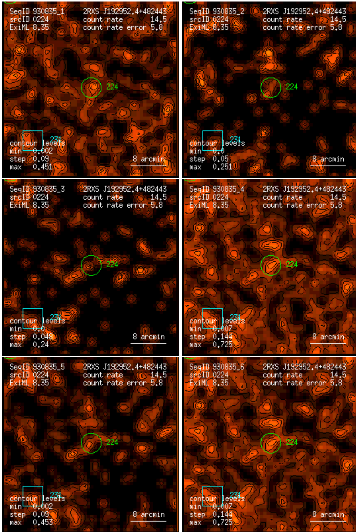
Figure 224: RASS 930835: detection 0224: band rate images, Gaussian filter: (1) PSPC channels 11 – 41, (2) 52 – 90, (3) 91 – 201, (4) 11 – 235, (5) 52 – 201, (6) 11 – 201. Broad band rates in counts/ks. Band rate contour levels in counts/ks/arcmin 2 .
