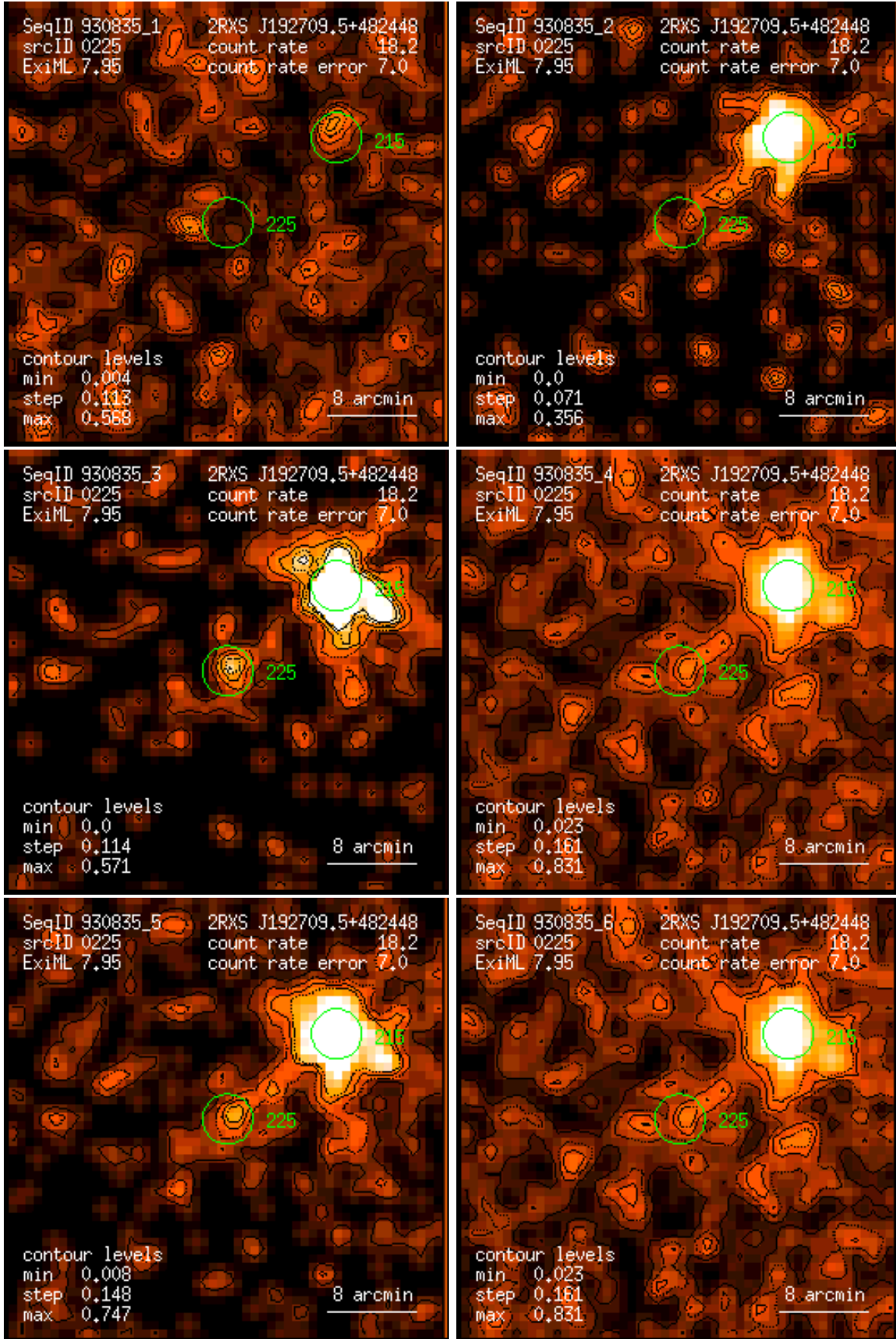
Figure 225: RASS 930835: detection 0225: band rate images, Gaussian filter: (1) PSPC channels 11 – 41, (2) 52 – 90, (3) 91 – 201, (4) 11 – 235, (5) 52 – 201, (6) 11 – 201. Broad band rates in counts/ks. Band rate contour levels in counts/ks/arcmin 2 .
