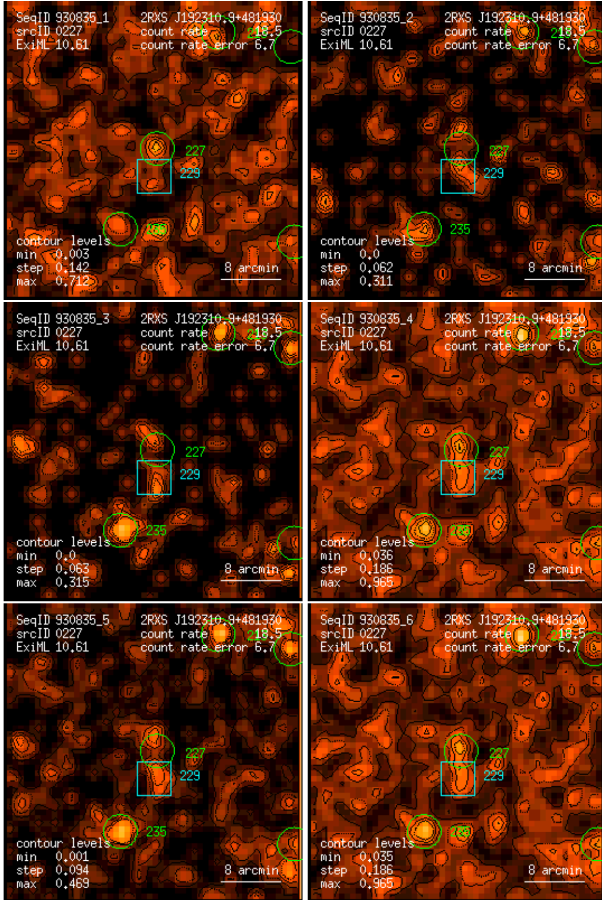
Figure 227: RASS 930835: detection 0227: band rate images, Gaussian filter: (1) PSPC channels 11 – 41, (2) 52 – 90, (3) 91 – 201, (4) 11 – 235, (5) 52 – 201, (6) 11 – 201. Broad band rates in counts/ks. Band rate contour levels in counts/ks/arcmin 2 .
