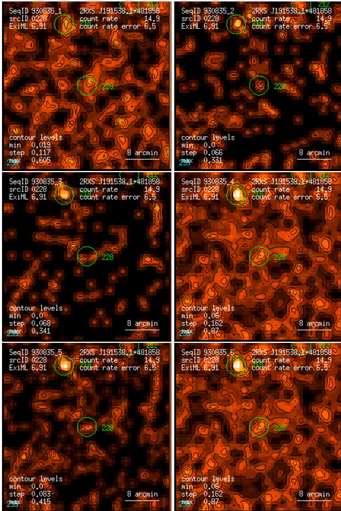
Figure 228: RASS 930835: detection 0228: band rate images, Gaussian filter: (1) PSPC channels 11 – 41, (2) 52 – 90, (3) 91 – 201, (4) 11 – 235, (5) 52 – 201, (6) 11 – 201. Broad band rates in counts/ks. Band rate contour levels in counts/ks/arcmin 2 .
