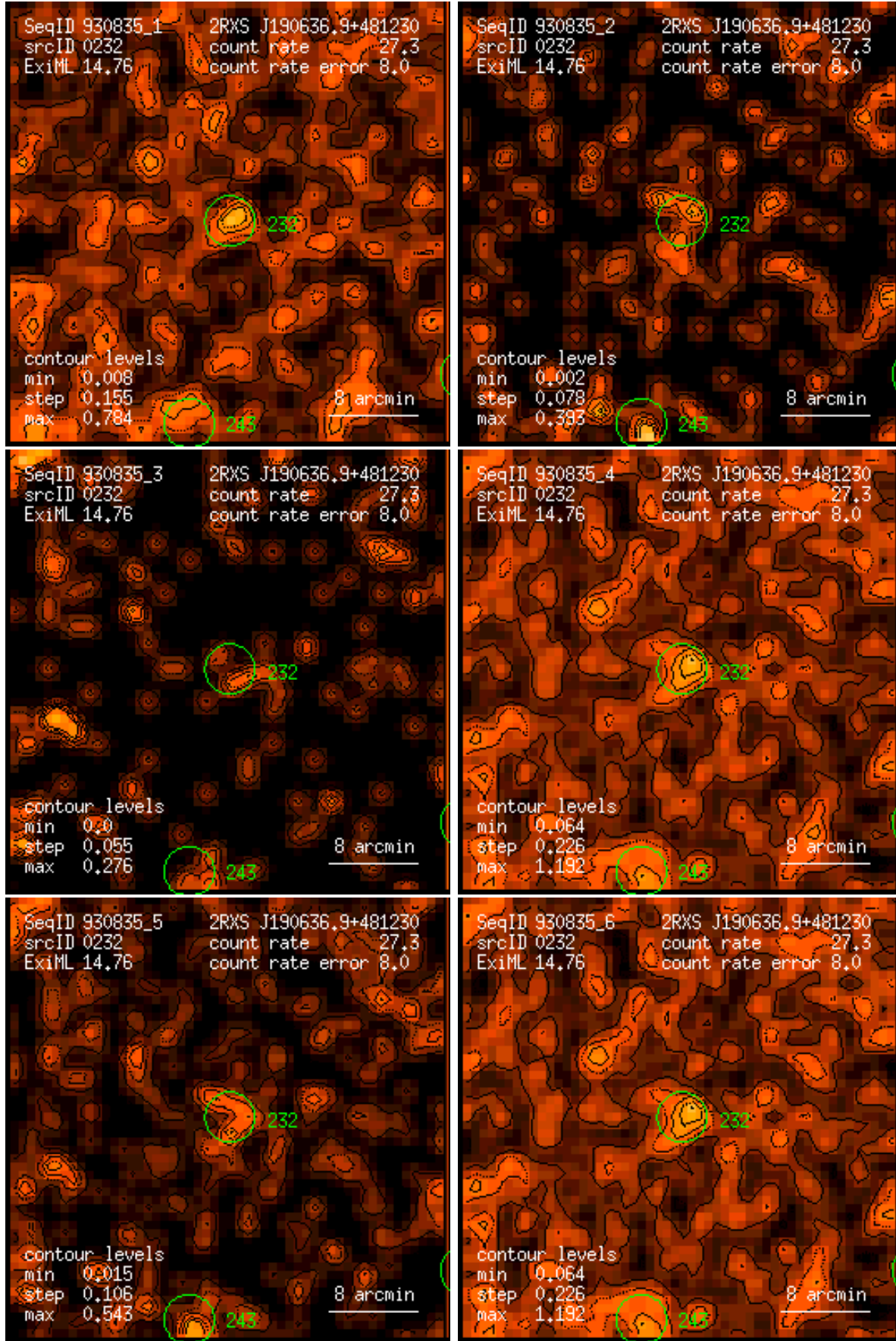
Figure 232: RASS 930835: detection 0232: band rate images, Gaussian filter: (1) PSPC channels 11 – 41, (2) 52 – 90, (3) 91 – 201, (4) 11 – 235, (5) 52 – 201, (6) 11 – 201. Broad band rates in counts/ks. Band rate contour levels in counts/ks/arcmin 2 .
