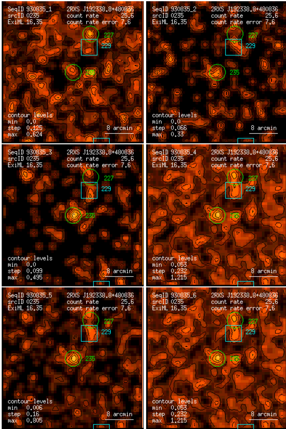
Figure 235: RASS 930835: detection 0235: band rate images, Gaussian filter: (1) PSPC channels 11 – 41, (2) 52 – 90, (3) 91 – 201, (4) 11 – 235, (5) 52 – 201, (6) 11 – 201. Broad band rates in counts/ks. Band rate contour levels in counts/ks/arcmin 2 .
