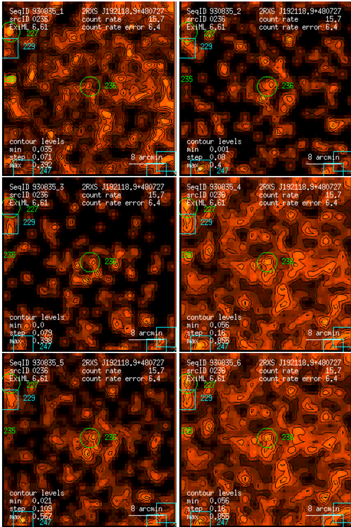
Figure 236: RASS 930835: detection 0236: band rate images, Gaussian filter: (1) PSPC channels 11 – 41, (2) 52 – 90, (3) 91 – 201, (4) 11 – 235, (5) 52 – 201, (6) 11 – 201. Broad band rates in counts/ks. Band rate contour levels in counts/ks/arcmin 2 .
