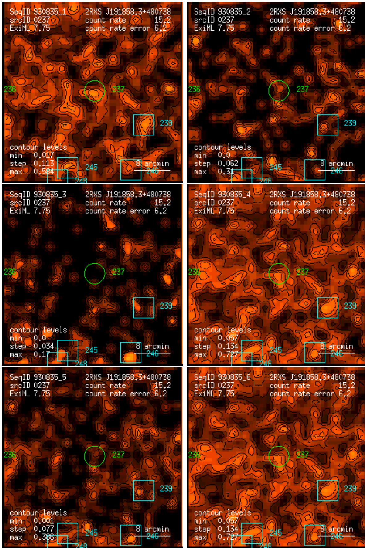
Figure 237: RASS 930835: detection 0237: band rate images, Gaussian filter: (1) PSPC channels 11 – 41, (2) 52 – 90, (3) 91 – 201, (4) 11 – 235, (5) 52 – 201, (6) 11 – 201. Broad band rates in counts/ks. Band rate contour levels in counts/ks/arcmin 2 .
