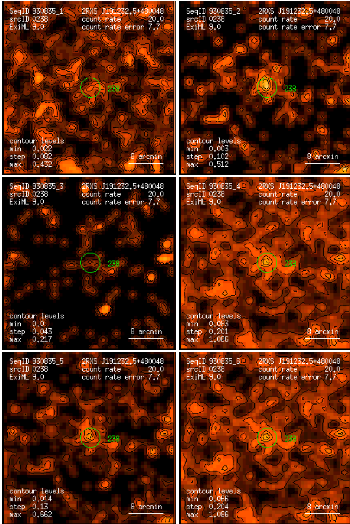
Figure 238: RASS 930835: detection 0238: band rate images, Gaussian filter: (1) PSPC channels 11 – 41, (2) 52 – 90, (3) 91 – 201, (4) 11 – 235, (5) 52 – 201, (6) 11 – 201. Broad band rates in counts/ks. Band rate contour levels in counts/ks/arcmin 2 .
