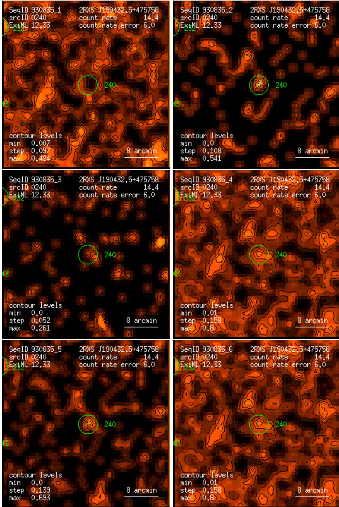
Figure 240: RASS 930835: detection 0240: band rate images, Gaussian filter: (1) PSPC channels 11 – 41, (2) 52 – 90, (3) 91 – 201, (4) 11 – 235, (5) 52 – 201, (6) 11 – 201. Broad band rates in counts/ks. Band rate contour levels in counts/ks/arcmin 2 .
