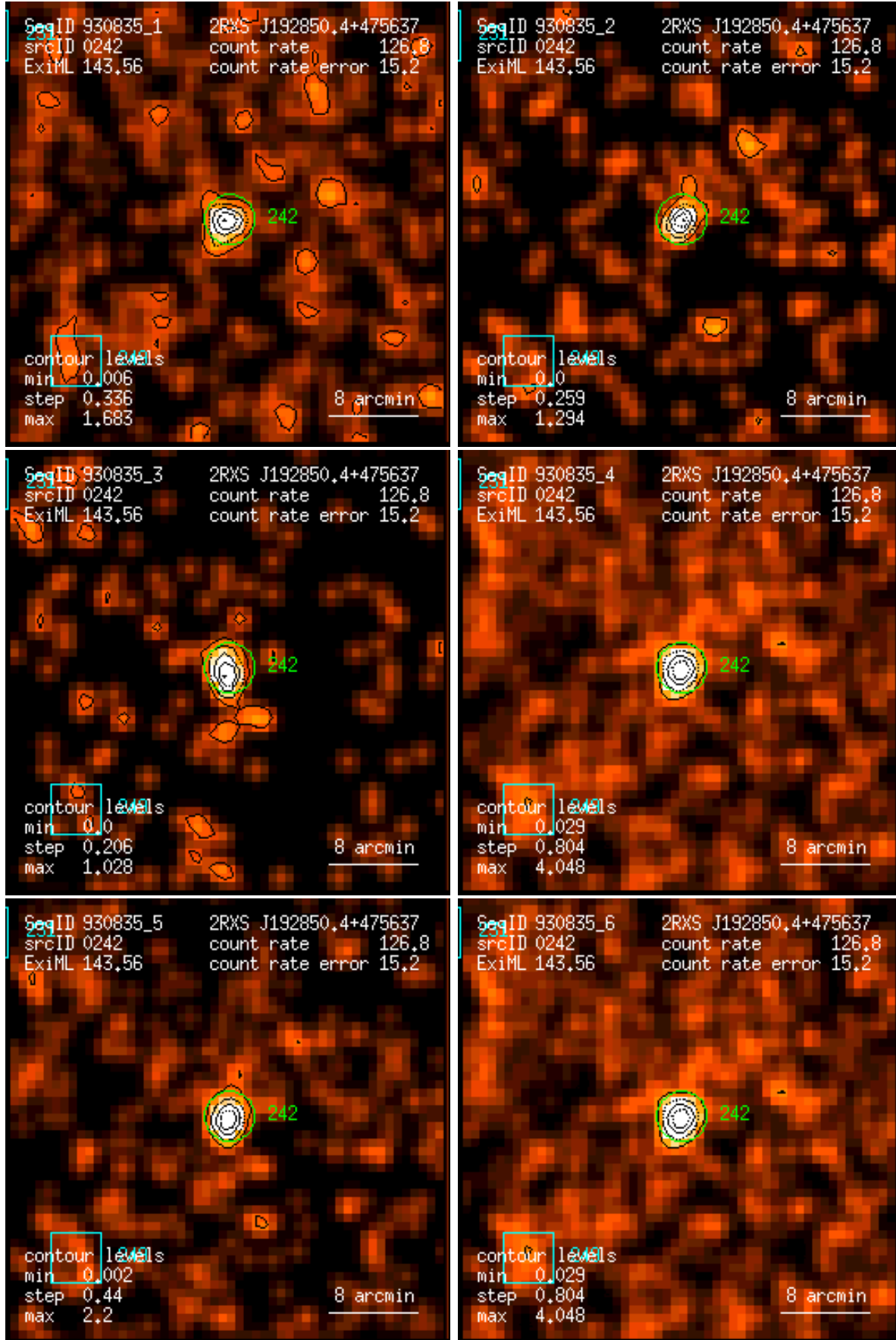
Figure 242: RASS 930835: detection 0242: band rate images, Gaussian filter: (1) PSPC channels 11 – 41, (2) 52 – 90, (3) 91 – 201, (4) 11 – 235, (5) 52 – 201, (6) 11 – 201. Broad band rates in counts/ks. Band rate contour levels in counts/ks/arcmin 2 .
