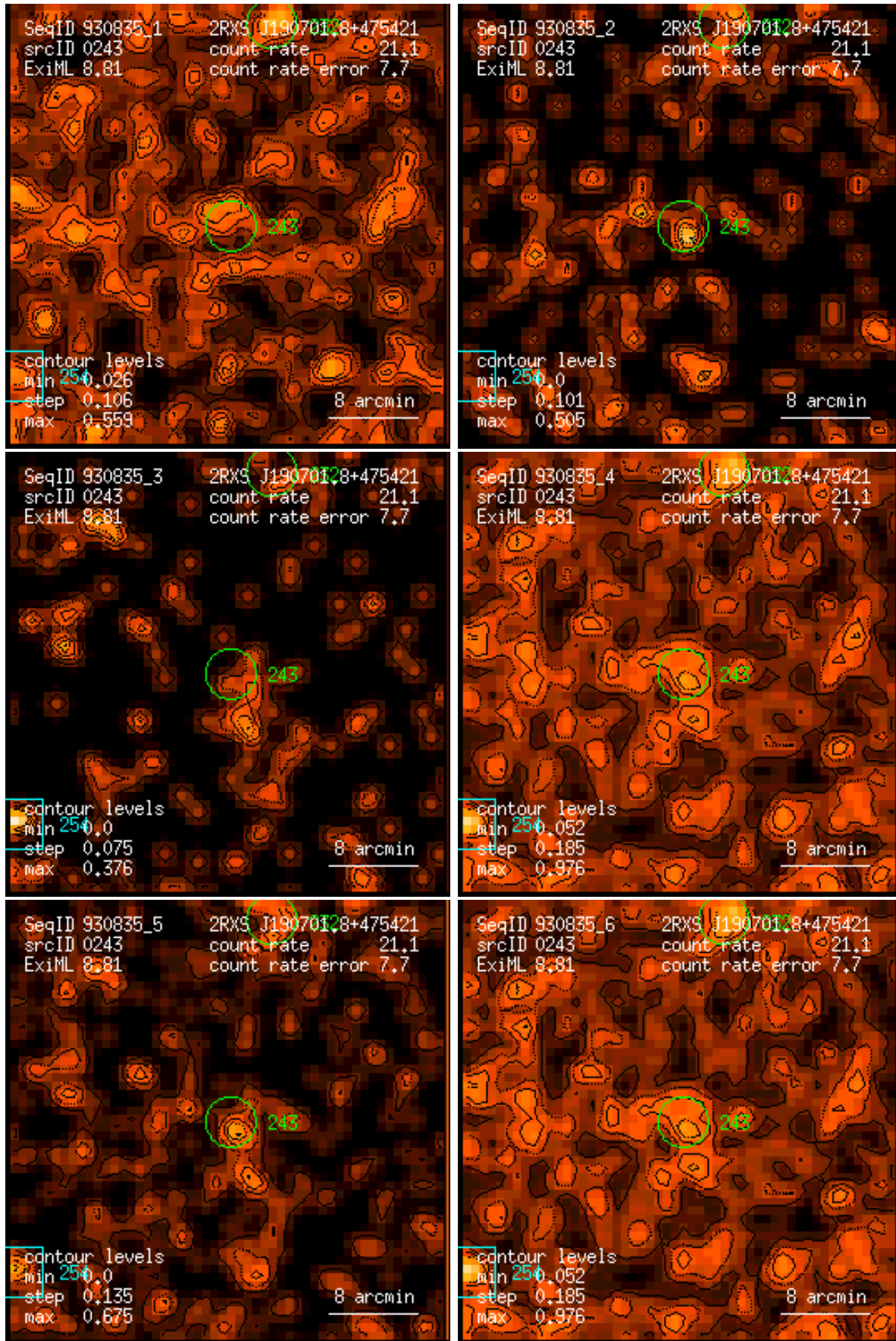
Figure 243: RASS 930835: detection 0243: band rate images, Gaussian filter: (1) PSPC channels 11 – 41, (2) 52 – 90, (3) 91 – 201, (4) 11 – 235, (5) 52 – 201, (6) 11 – 201. Broad band rates in counts/ks. Band rate contour levels in counts/ks/arcmin 2 .
