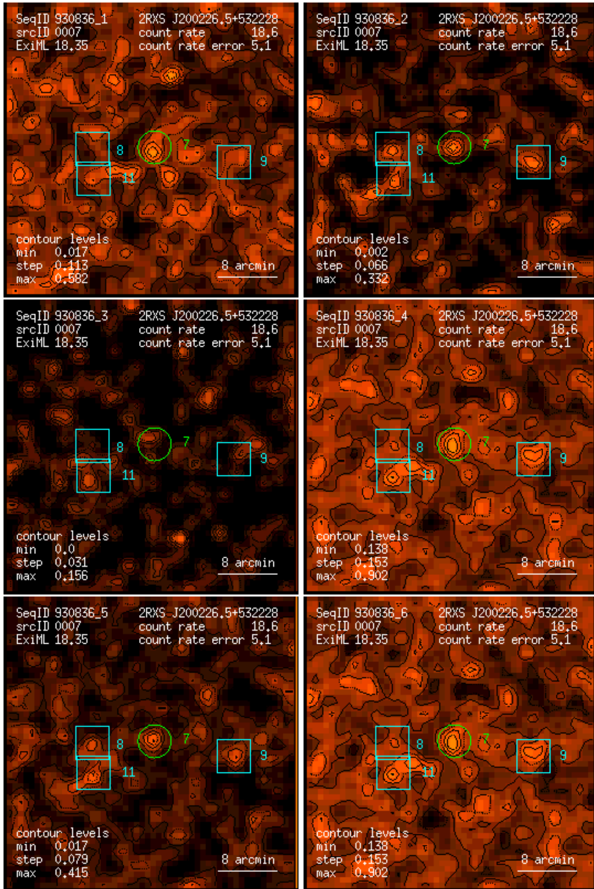
Figure 7: RASS 930836: detection 0007: band rate images, Gaussian filter: (1) PSPC channels 11 – 41, (2) 52 – 90, (3) 91 – 201, (4) 11 – 235, (5) 52 – 201, (6) 11 – 201. Broad band rates in counts/ks. Band rate contour levels in counts/ks/arcmin 2 .
