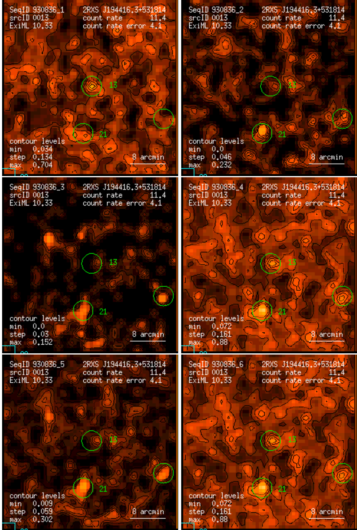
Figure 13: RASS 930836: detection 0013: band rate images, Gaussian filter: (1) PSPC channels 11 – 41, (2) 52 – 90, (3) 91 – 201, (4) 11 – 235, (5) 52 – 201, (6) 11 – 201. Broad band rates in counts/ks. Band rate contour levels in counts/ks/arcmin 2 .
