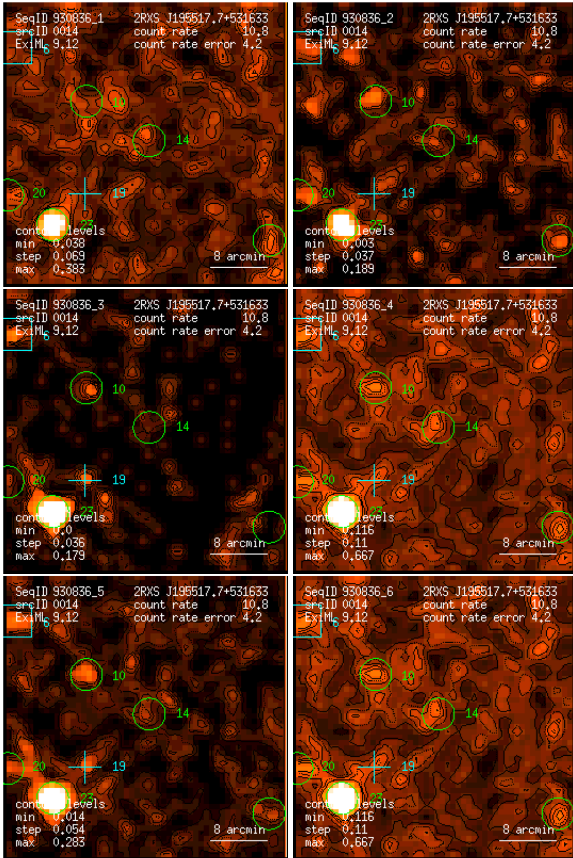
Figure 14: RASS 930836: detection 0014: band rate images, Gaussian filter: (1) PSPC channels 11 – 41, (2) 52 – 90, (3) 91 – 201, (4) 11 – 235, (5) 52 – 201, (6) 11 – 201. Broad band rates in counts/ks. Band rate contour levels in counts/ks/arcmin 2 .
