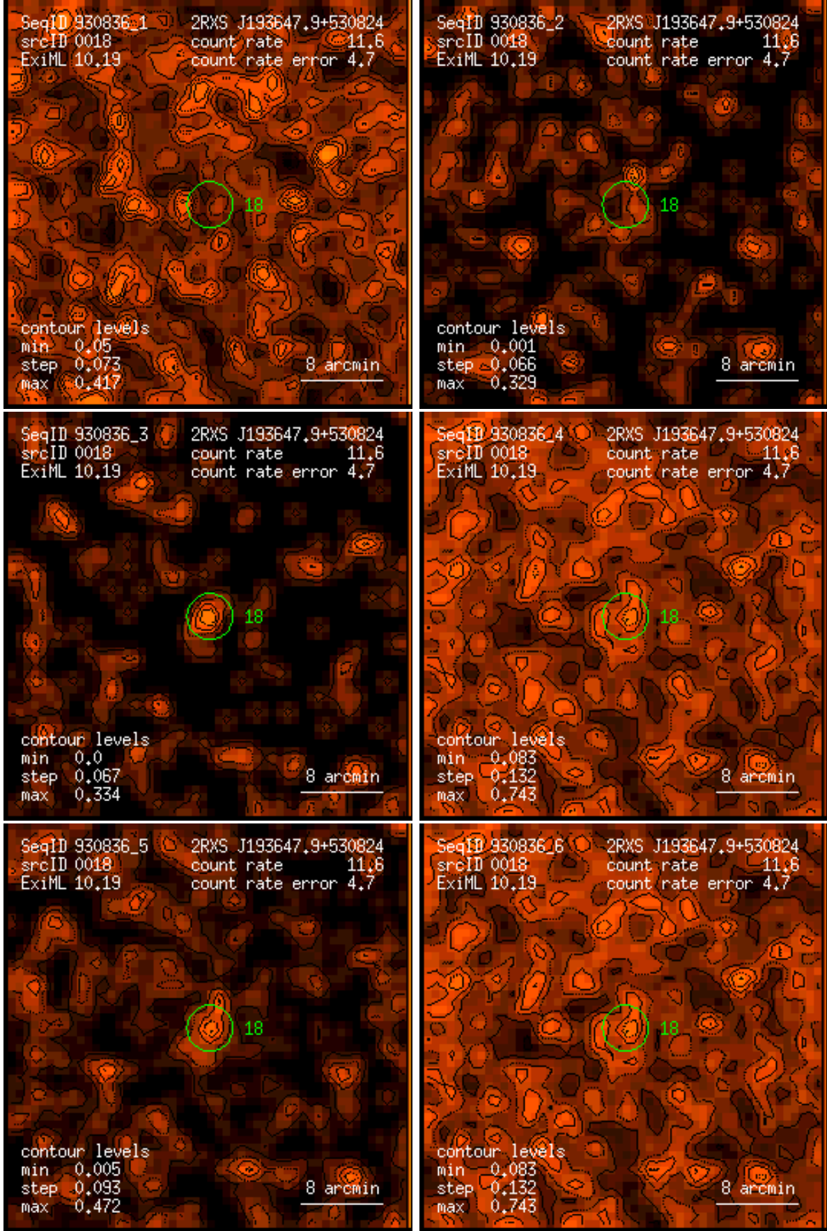
Figure 18: RASS 930836: detection 0018: band rate images, Gaussian filter: (1) PSPC channels 11 – 41, (2) 52 – 90, (3) 91 – 201, (4) 11 – 235, (5) 52 – 201, (6) 11 – 201. Broad band rates in counts/ks. Band rate contour levels in counts/ks/arcmin 2 .
