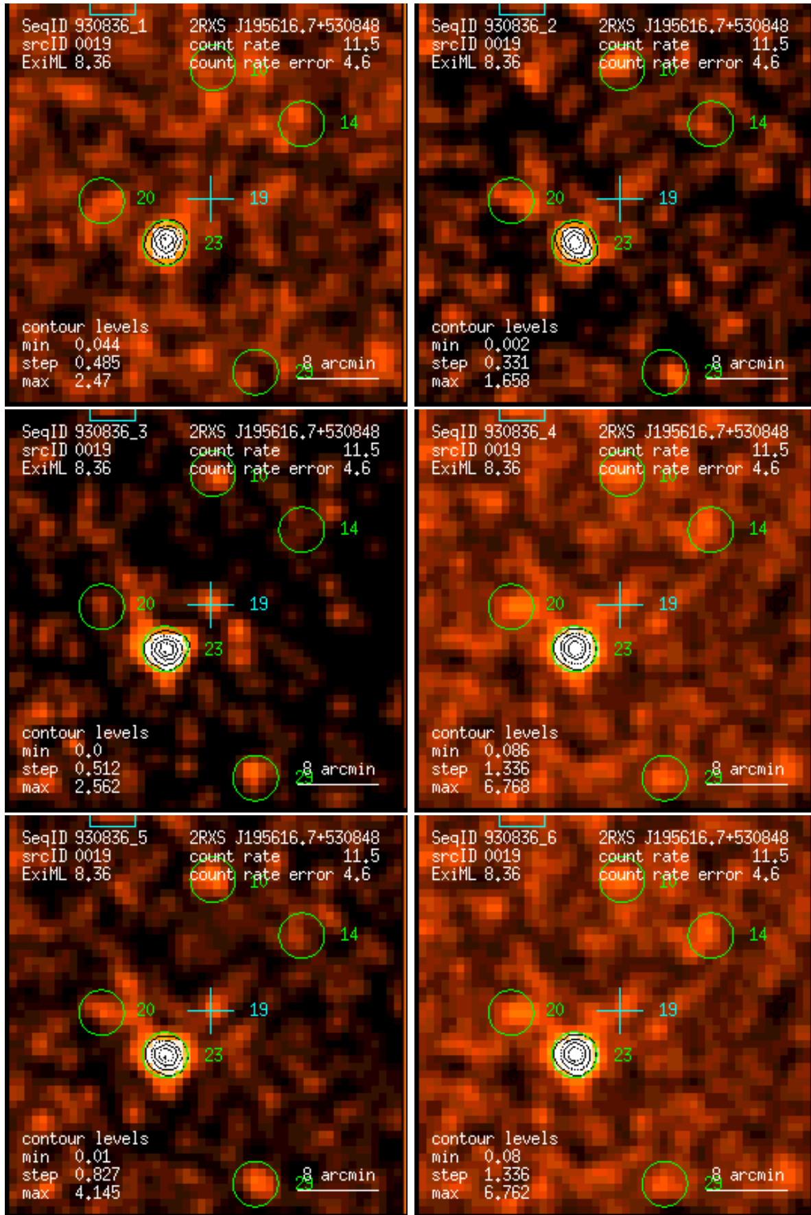
Figure 19: RASS 930836: detection 0019: band rate images, Gaussian filter: (1) PSPC channels 11 – 41, (2) 52 – 90, (3) 91 – 201, (4) 11 – 235, (5) 52 – 201, (6) 11 – 201. Broad band rates in counts/ks. Band rate contour levels in counts/ks/arcmin 2 .
