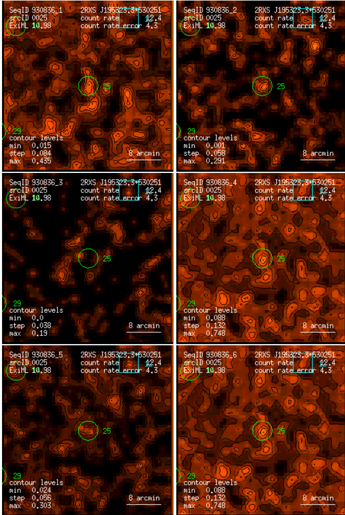
Figure 25: RASS 930836: detection 0025: band rate images, Gaussian filter: (1) PSPC channels 11 – 41, (2) 52 – 90, (3) 91 – 201, (4) 11 – 235, (5) 52 – 201, (6) 11 – 201. Broad band rates in counts/ks. Band rate contour levels in counts/ks/arcmin 2 .
