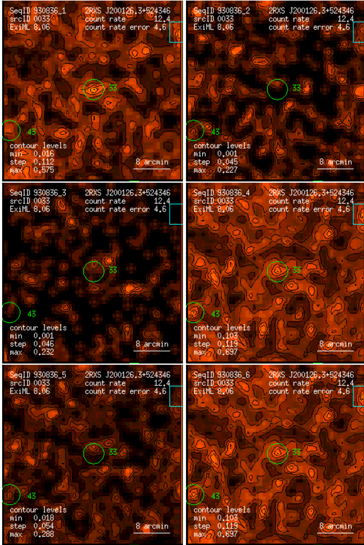
Figure 33: RASS 930836: detection 0033: band rate images, Gaussian filter: (1) PSPC channels 11 – 41, (2) 52 – 90, (3) 91 – 201, (4) 11 – 235, (5) 52 – 201, (6) 11 – 201. Broad band rates in counts/ks. Band rate contour levels in counts/ks/arcmin 2 .
