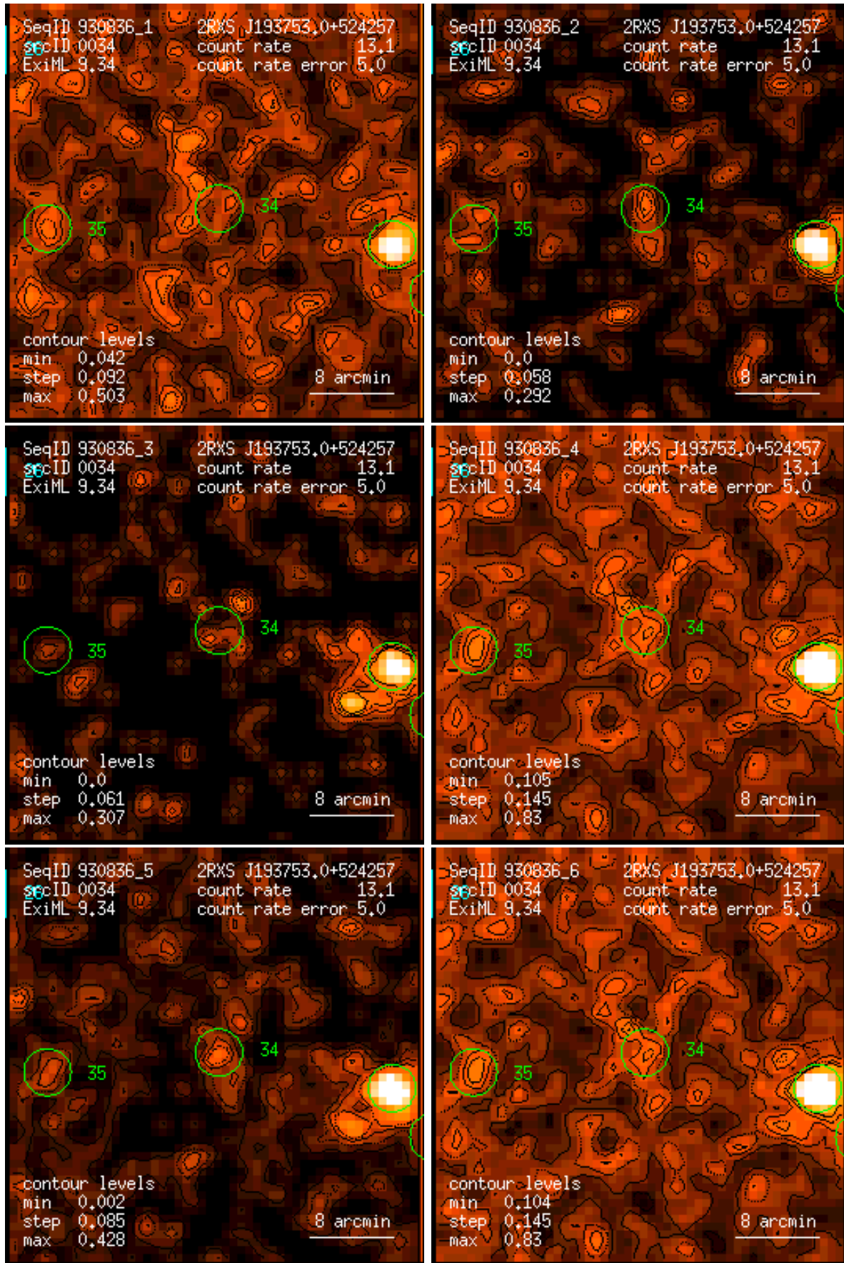
Figure 34: RASS 930836: detection 0034: band rate images, Gaussian filter: (1) PSPC channels 11 – 41, (2) 52 – 90, (3) 91 – 201, (4) 11 – 235, (5) 52 – 201, (6) 11 – 201. Broad band rates in counts/ks. Band rate contour levels in counts/ks/arcmin 2 .
