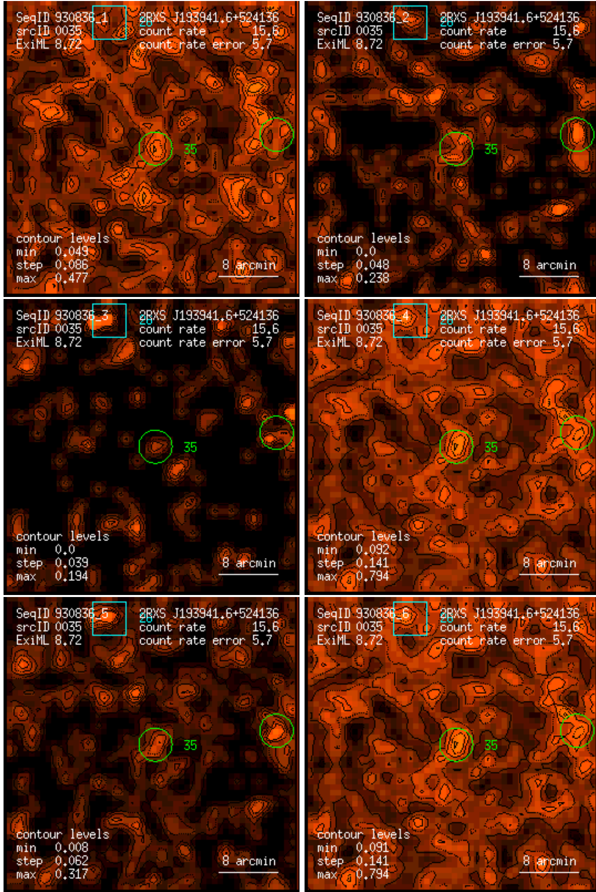
Figure 35: RASS 930836: detection 0035: band rate images, Gaussian filter: (1) PSPC channels 11 – 41, (2) 52 – 90, (3) 91 – 201, (4) 11 – 235, (5) 52 – 201, (6) 11 – 201. Broad band rates in counts/ks. Band rate contour levels in counts/ks/arcmin 2 .
