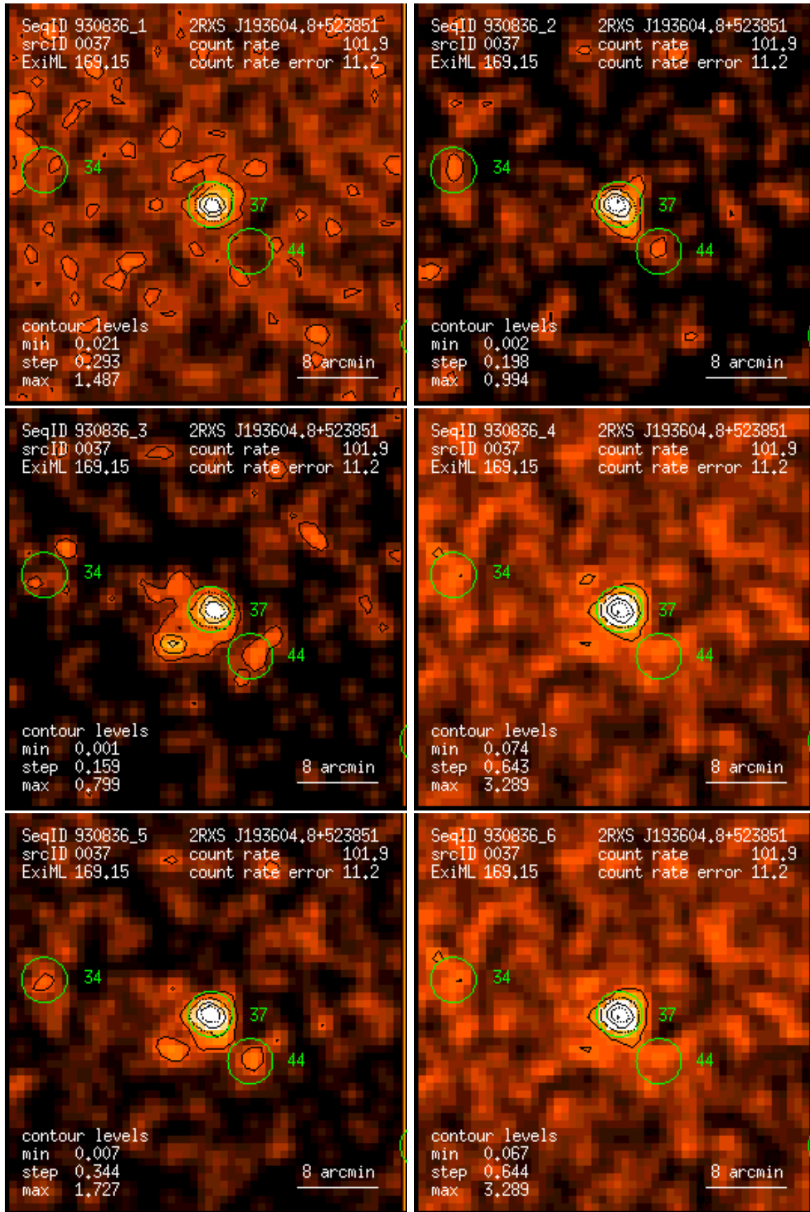
Figure 37: RASS 930836: detection 0037: band rate images, Gaussian filter: (1) PSPC channels 11 – 41, (2) 52 – 90, (3) 91 – 201, (4) 11 – 235, (5) 52 – 201, (6) 11 – 201. Broad band rates in counts/ks. Band rate contour levels in counts/ks/arcmin 2 .
