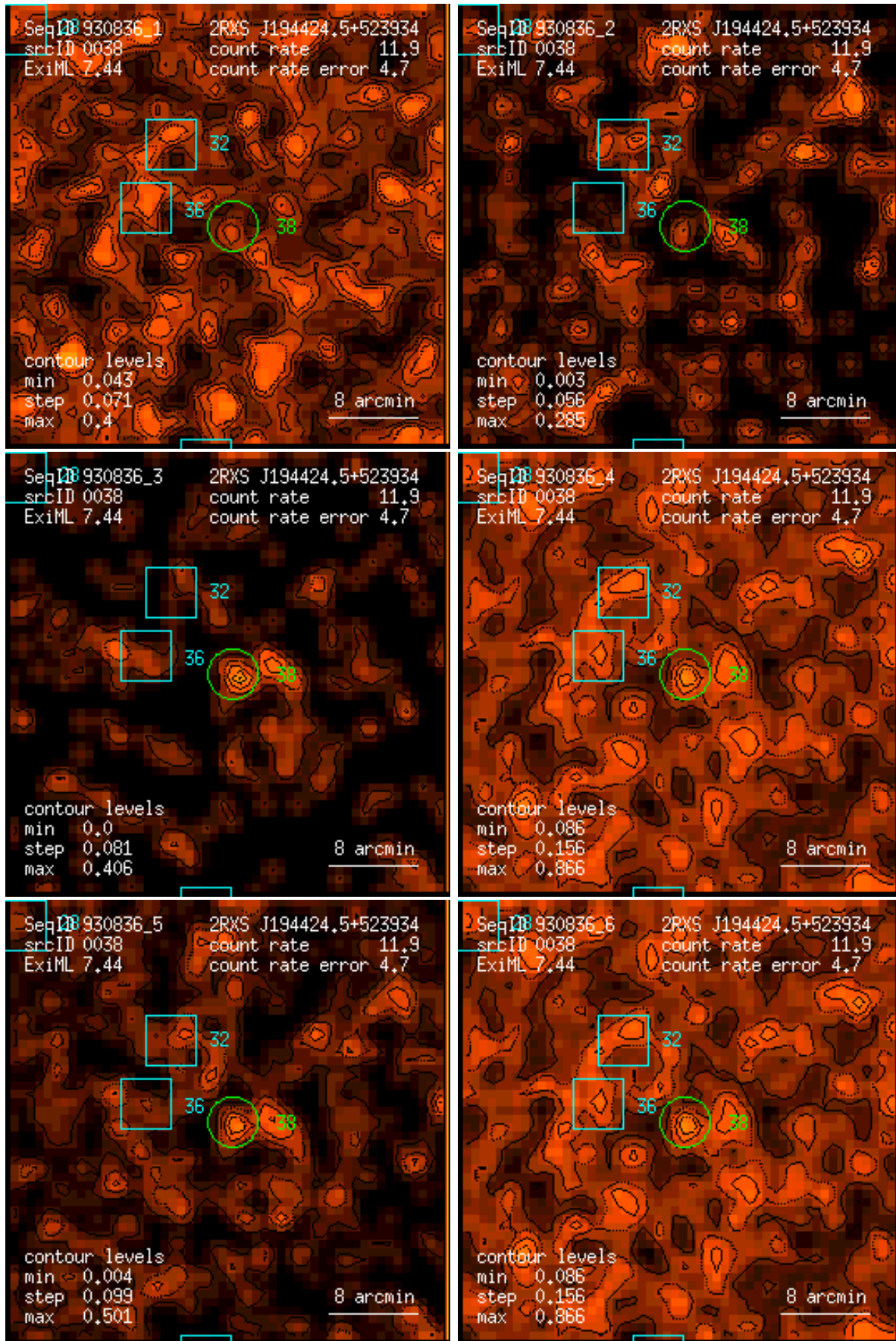
Figure 38: RASS 930836: detection 0038: band rate images, Gaussian filter: (1) PSPC channels 11 – 41, (2) 52 – 90, (3) 91 – 201, (4) 11 – 235, (5) 52 – 201, (6) 11 – 201. Broad band rates in counts/ks. Band rate contour levels in counts/ks/arcmin 2 .
