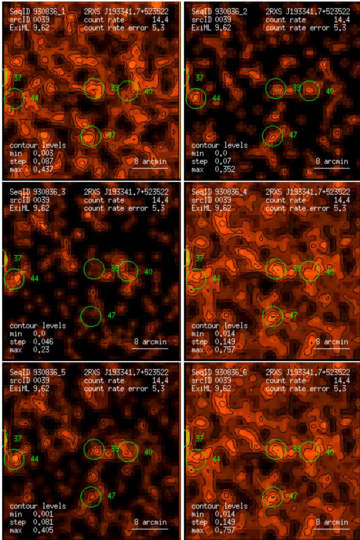
Figure 39: RASS 930836: detection 0039: band rate images, Gaussian filter: (1) PSPC channels 11 – 41, (2) 52 – 90, (3) 91 – 201, (4) 11 – 235, (5) 52 – 201, (6) 11 – 201. Broad band rates in counts/ks. Band rate contour levels in counts/ks/arcmin 2 .
