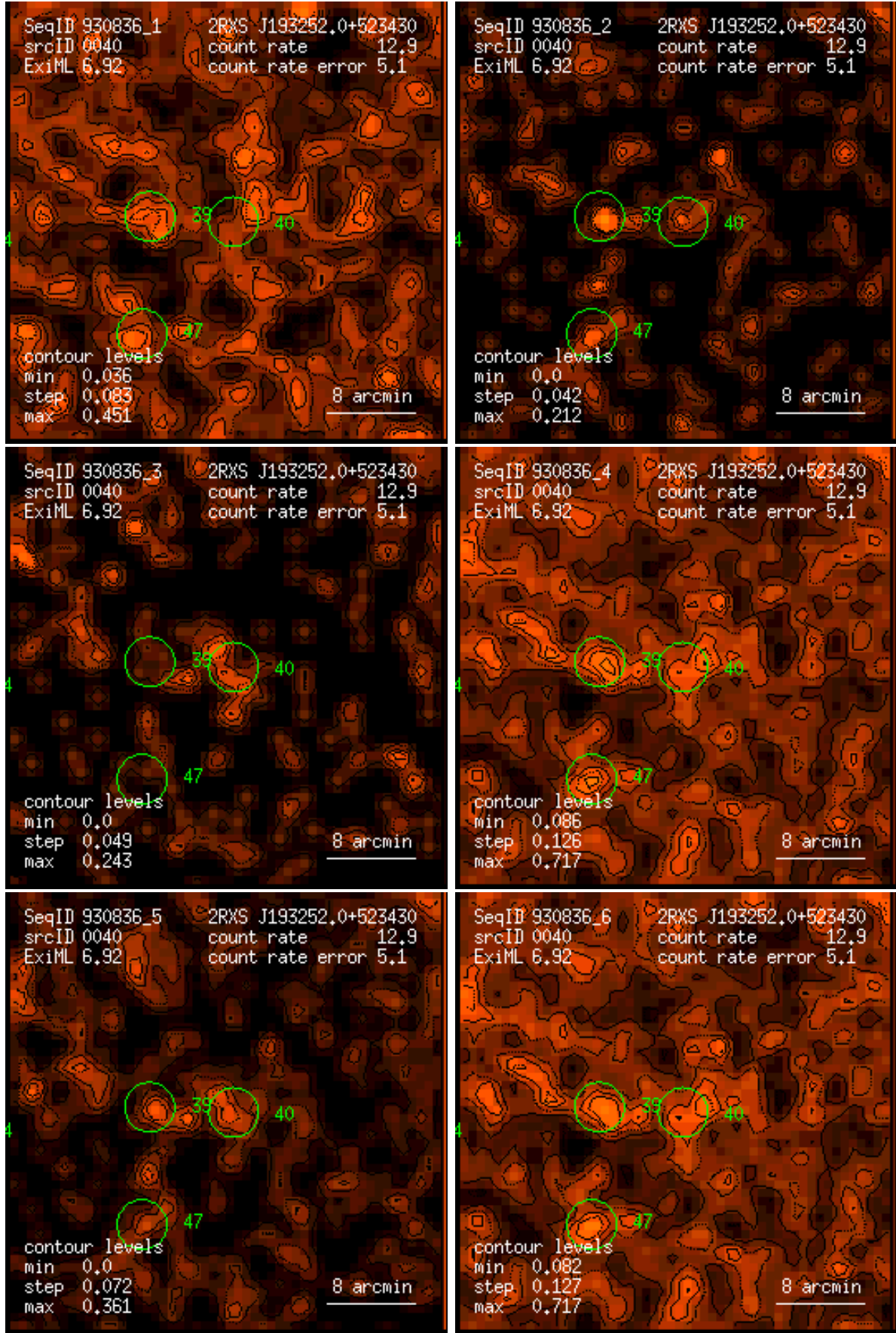
Figure 40: RASS 930836: detection 0040: band rate images, Gaussian filter: (1) PSPC channels 11 – 41, (2) 52 – 90, (3) 91 – 201, (4) 11 – 235, (5) 52 – 201, (6) 11 – 201. Broad band rates in counts/ks. Band rate contour levels in counts/ks/arcmin 2 .
