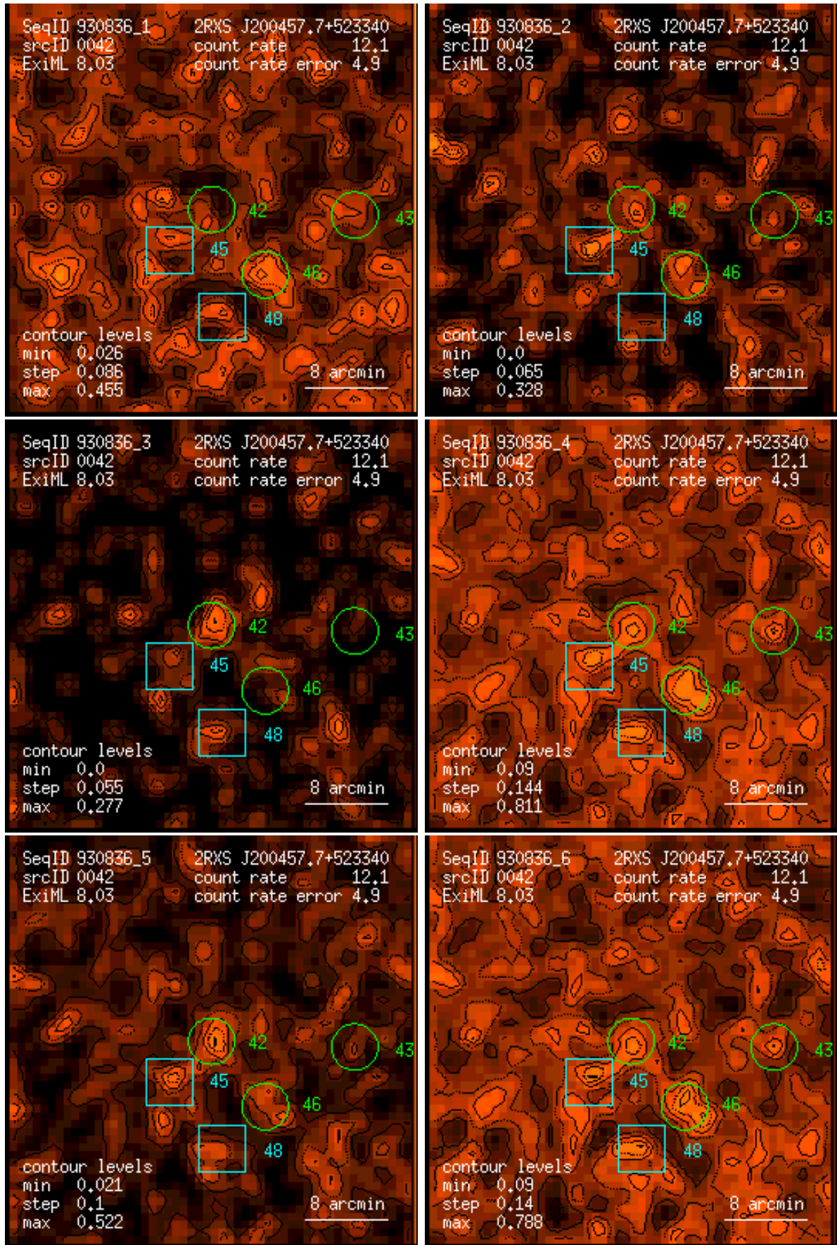
Figure 42: RASS 930836: detection 0042: band rate images, Gaussian filter: (1) PSPC channels 11 – 41, (2) 52 – 90, (3) 91 – 201, (4) 11 – 235, (5) 52 – 201, (6) 11 – 201. Broad band rates in counts/ks. Band rate contour levels in counts/ks/arcmin 2 .
