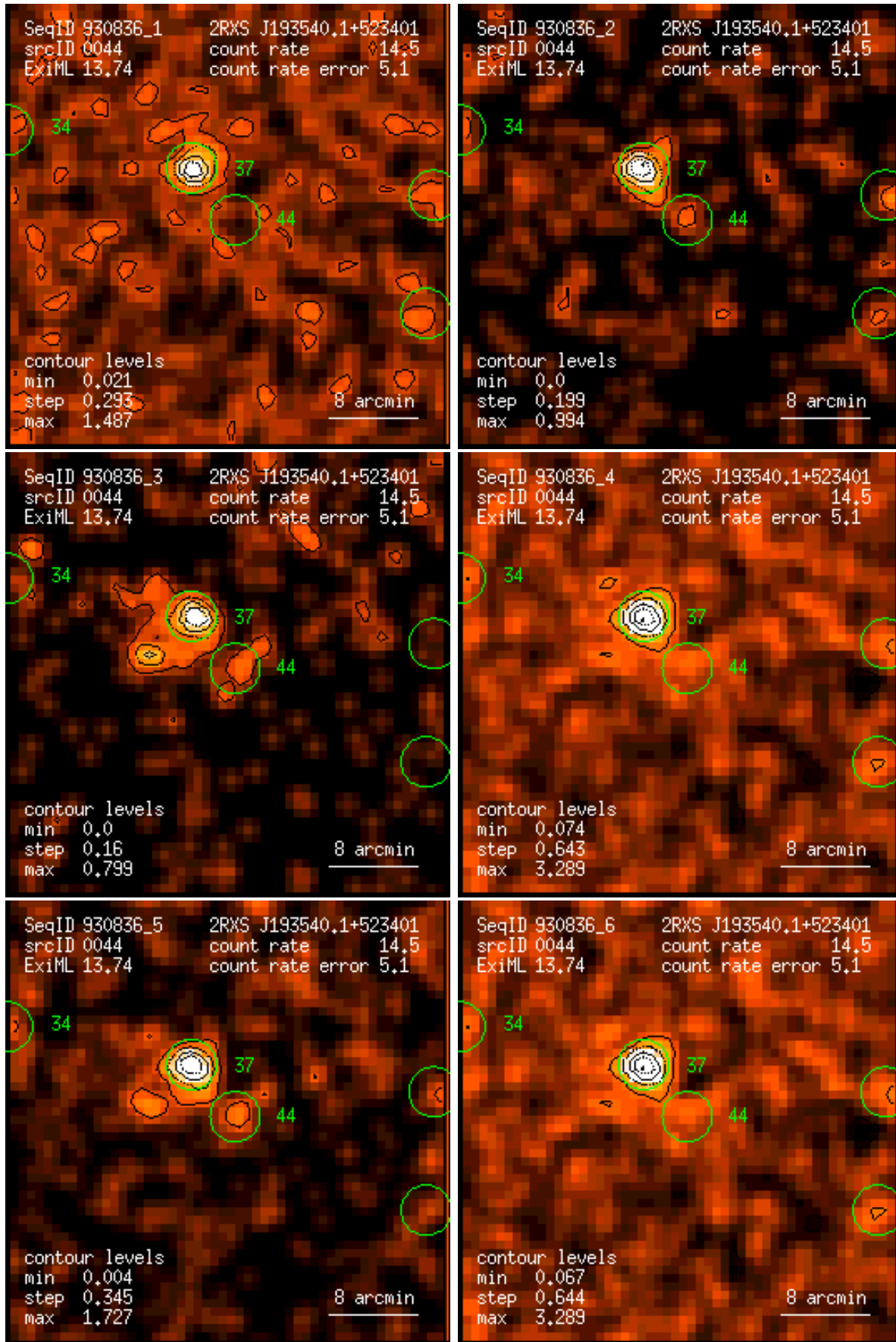
Figure 44: RASS 930836: detection 0044: band rate images, Gaussian filter: (1) PSPC channels 11 – 41, (2) 52 – 90, (3) 91 – 201, (4) 11 – 235, (5) 52 – 201, (6) 11 – 201. Broad band rates in counts/ks. Band rate contour levels in counts/ks/arcmin 2 .
