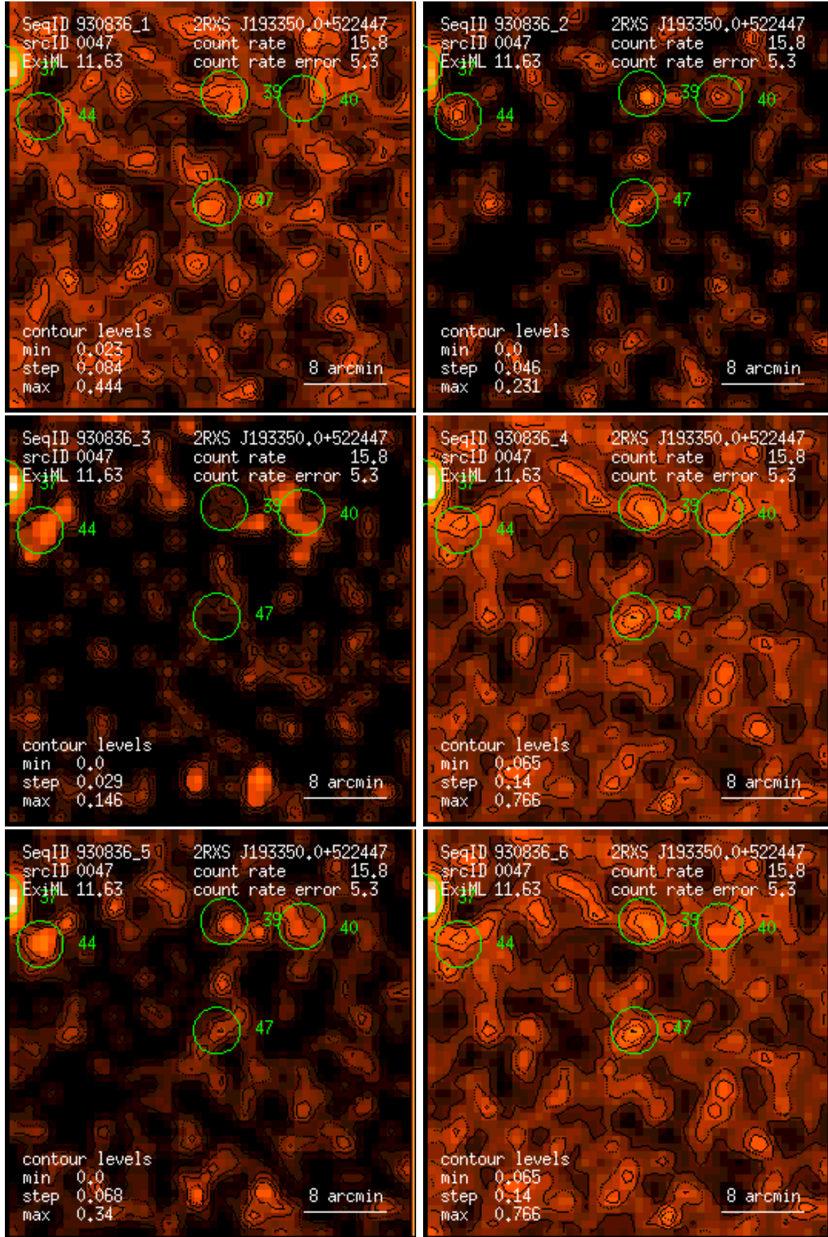
Figure 47: RASS 930836: detection 0047: band rate images, Gaussian filter: (1) PSPC channels 11 – 41, (2) 52 – 90, (3) 91 – 201, (4) 11 – 235, (5) 52 – 201, (6) 11 – 201. Broad band rates in counts/ks. Band rate contour levels in counts/ks/arcmin 2 .
